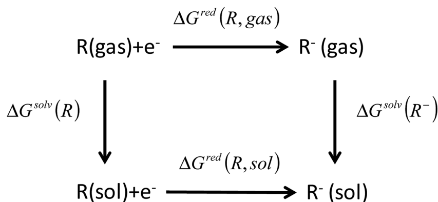
Fig. 2 Thermodynamic cycle used to calculate the equilibrium redox potential in the condensed phase. 33,34
