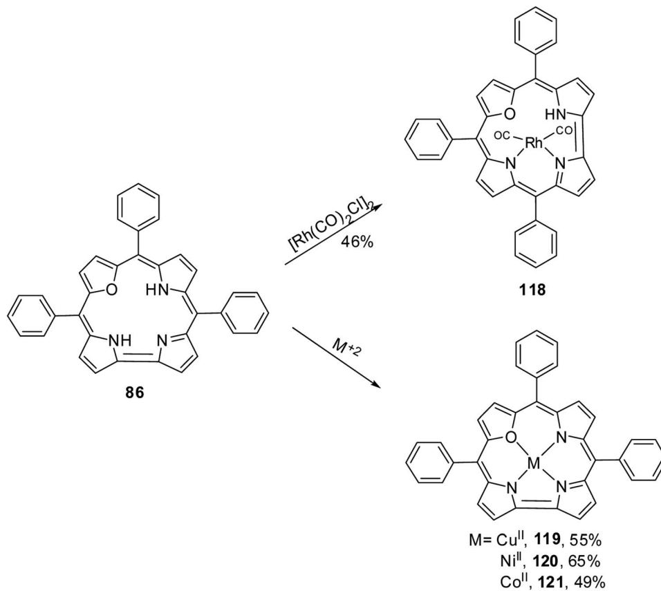
Scheme 27 Synthesis of metal derivatives of 22-oxacorrrole 118–121.
