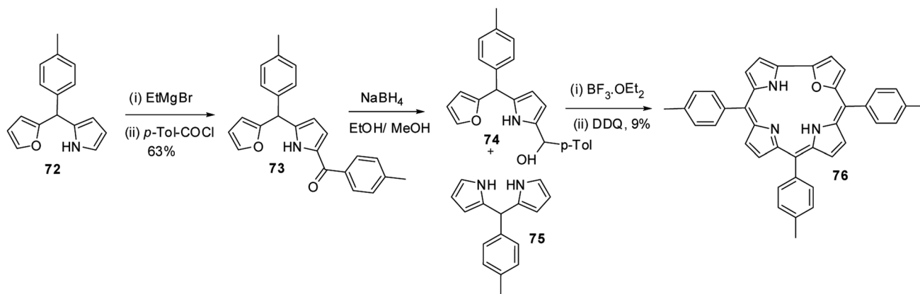
Scheme 18 Synthesis of meso -substituted 21-oxacorrole 76 .
