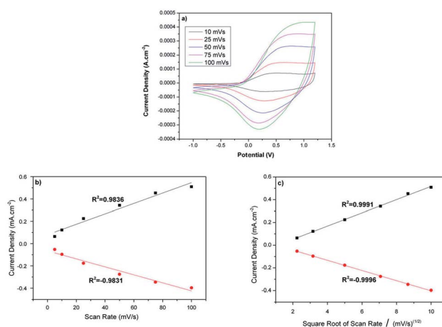
Fig. 3 (a) Cyclic voltammogram of PEDOT nanofibers in 0.1\text{ M NBu}_4\text{PF}_6/\text{ACN} at various scan rates, and plots of the anodic and cathodic peak current densities vs. (b) the scan rate, (c) the square root of the scan rate.
