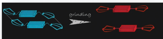
Fig. 1 (Top) The molecular structures of compounds 1 and 2 . (Bottom) An illustration of the MFC mechanism based on the planarization of the molecular conformation.
