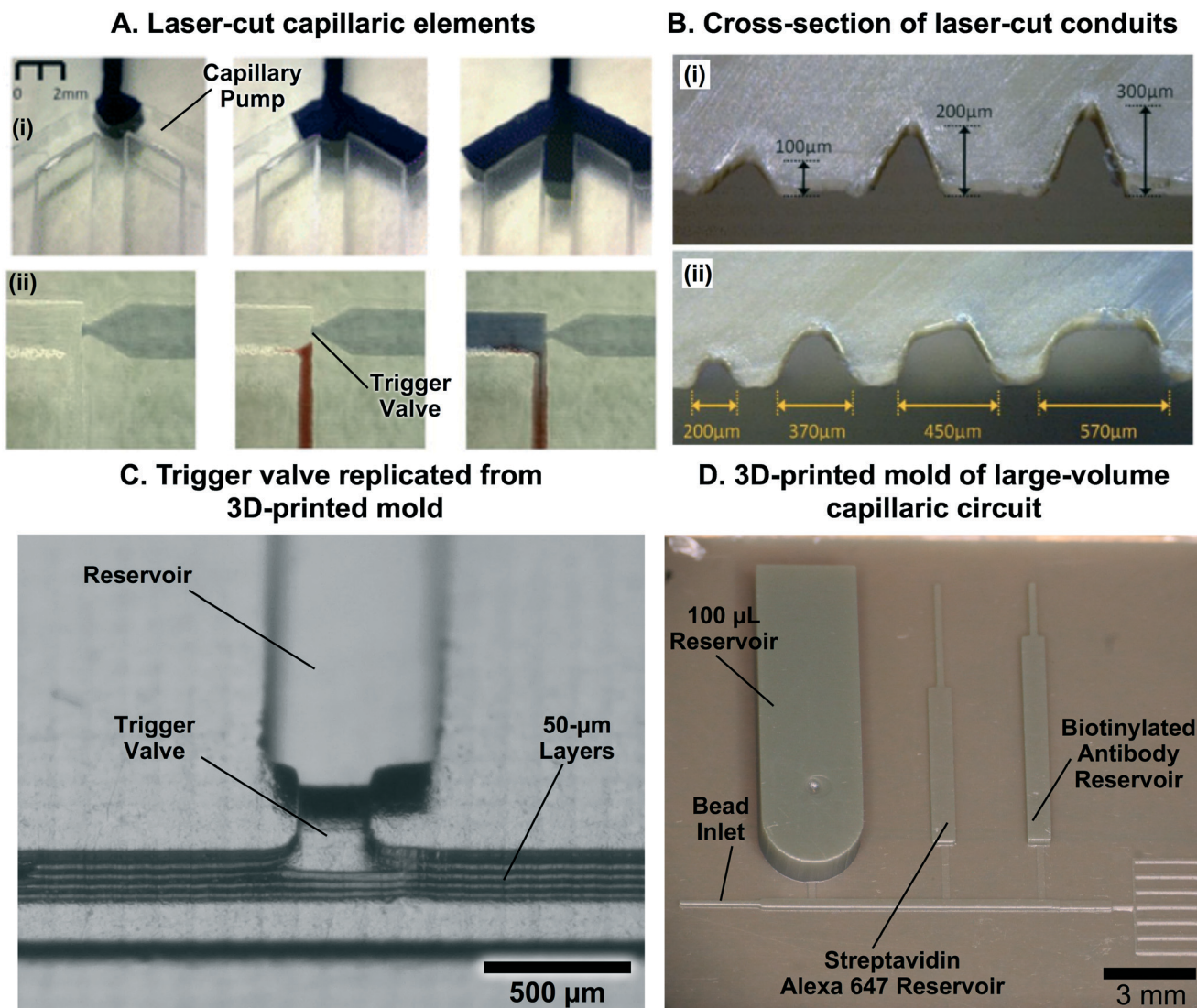
Fig. 13 Rapid prototyping of capillalic components and circuits using CO 2 laser cutting and 3D-printing. (A) Capillalic components fabricated by CO 2 laser cutting. (i) Capillary pump, (ii) trigger valves. (B) Cross-sections of microchannels fabricated by laser cutting. Smaller microchannels (i) have a triangular Gaussian profile that reflects the shape of the laser beam, while (ii) wider microchannels have a more rectangular shape due to repeated scanning of the laser. (C) Front view of 3D-printed trigger valve showing inherent layer-by-layer structure. (D) 3D-printed mold of CC for bacteria detection showing physical realization of structures. Adapted with permission from: (A) ref. 42 © 2013 Springer-Verlag, (B) ref. 42 © 2013 Springer-Verlag Berlin Heidelberg, (C) ref. 44 © 2016 Royal Society of Chemistry, (D) ref. 45 © 2017 American Chemical Society.
