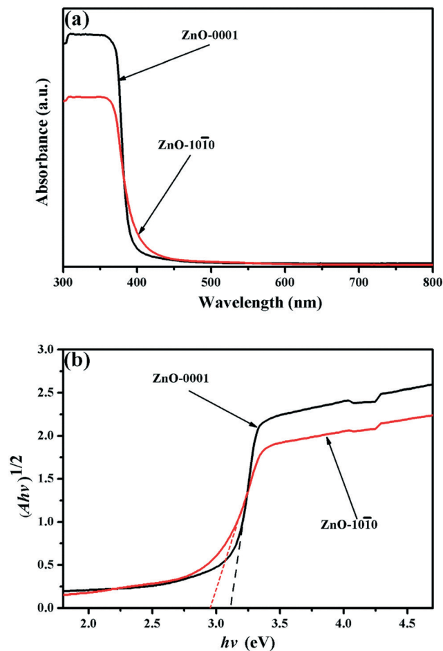
Fig. 5 (a) UV-vis DRS spectra and (b) plots of (A\hbar\nu)^{1/2} versus photon energy ( \hbar\nu ) of ZnO-0001 and ZnO-10 \bar{1}0 .
