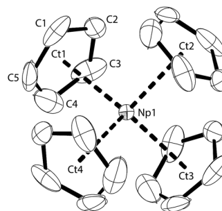
Fig. 1 Thermal ellipsoid drawing (50% probability for non-H atoms) of \text{NpCp}_4 in the solid state. H atoms omitted. Selected bond lengths [Å] and angles [°] for \text{NpCp}_4 : \text{Np1-Ct} 2.551(2), \text{Np1-C} 2.78(1) to 2.83(1), \text{Ct-Np1-Ct} 109.4(2).
