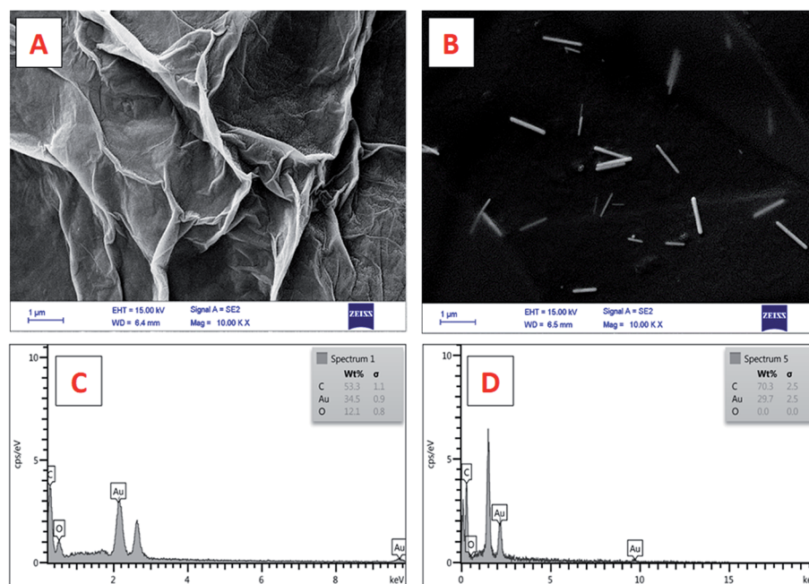
Fig. 1 FESEM images of the SPCE electrode surface modified with (A) graphene oxide and (B) gold nanowires decorated on the graphene oxide. EDX analysis of the modified SPCE electrode surface (C) before (AuNWs + GO) and (D) after electrochemical reduction of the graphene oxide decorated with the gold nanowires (AuNWs + ERGO).
