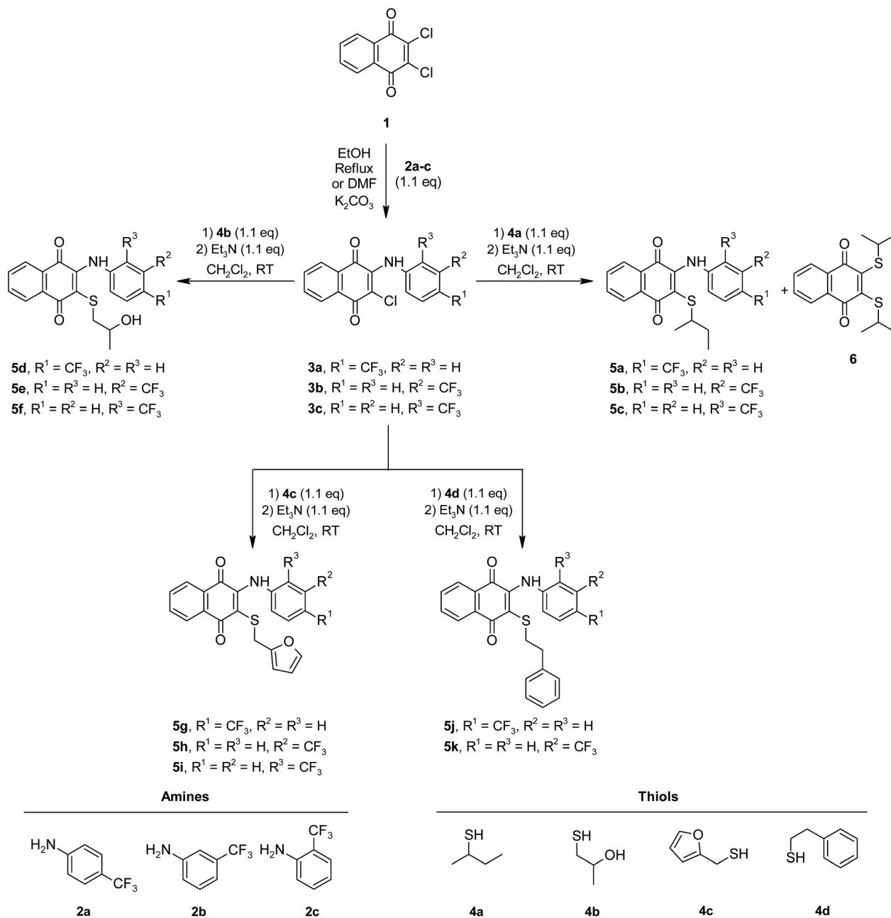
Scheme 1 Synthetic pathway for the preparation of new sulfanyl 1,4-naphthoquinone derivatives substituted with arylamines containing the -\text{CF}_3 at o -, m -, and p -positions.
