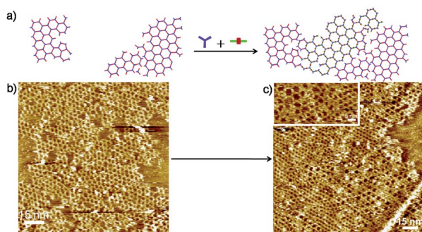
Fig. 6 (a) A schematic diagram of the formation of 2DP hetero-structure on the surface. STM images of the submonolayer of 2DP 1+3 (b) and in situ synthesized hetero-structure of 2DP 1+3 /2D 1+4 (c) at the octanoic acid/HOPG interface. Imaging conditions: (b) I_{\text{set}} = 28 pA, V_{\text{bias}} = 0.68 V; (c) and inset I_{\text{set}} = 27 pA, V_{\text{bias}} = 0.52 V.
