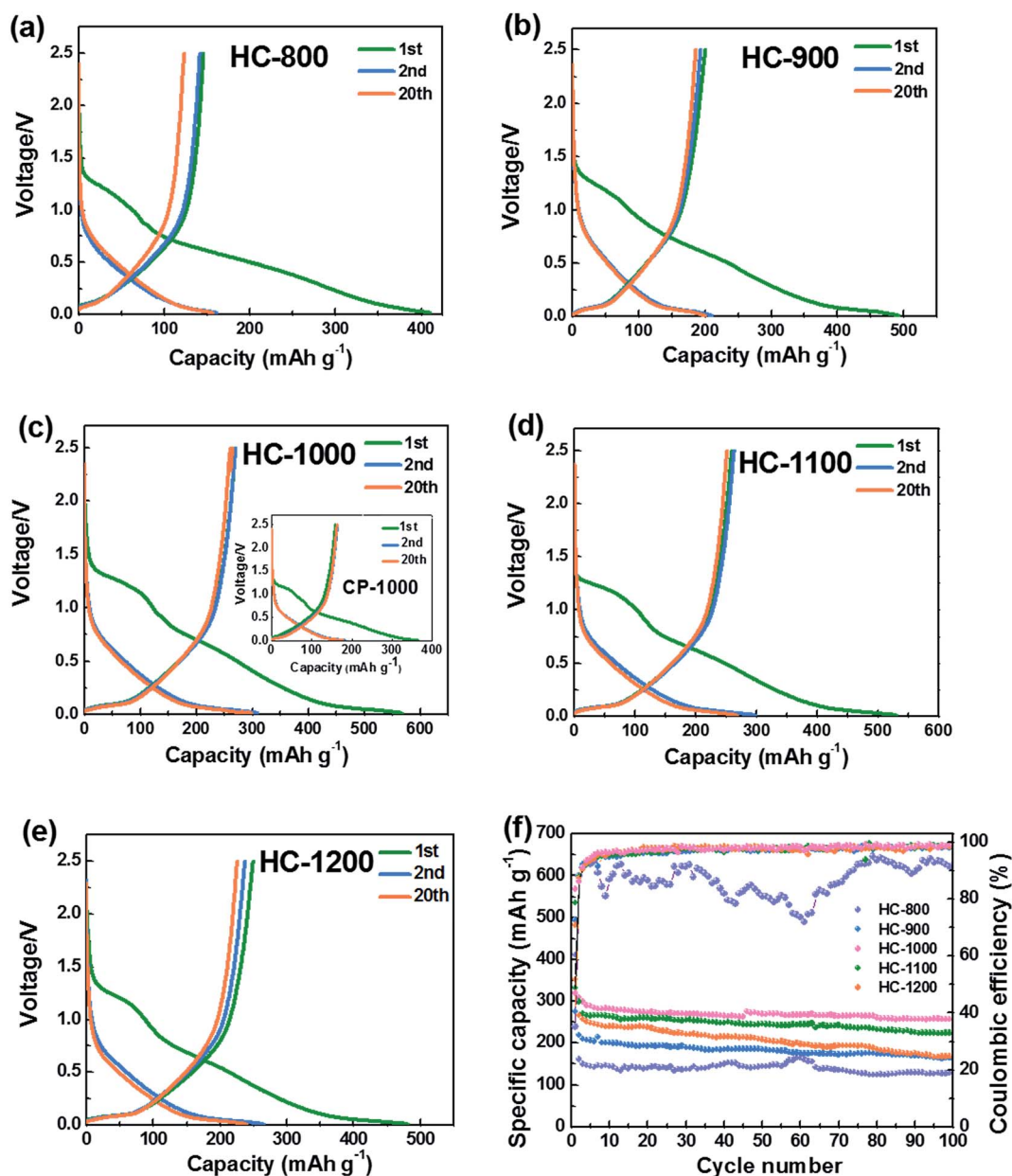
Fig. 5 Discharge–charge profiles of hard carbons at 20 \text{mA g}^{-1} (a) HC-800 (b) HC-900 (c) HC-1000 and CP-1000 (d) HC-1100, and (e) HC-1200, (f) cycling performance of HC electrodes tested at 20 \text{mA g}^{-1} , the voltage range is between 0.01 and 2.5 V.
