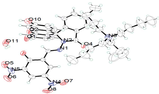
Fig. 7 Molecular structure (ORTEP) of FKCN at 40% probability level.
