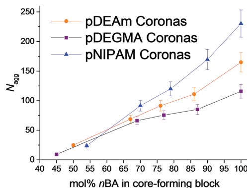
Fig. 2 Variation in the particles' N_{\text{agg}} with the molar fraction of hydrophobic n BA in the core-forming block, as determined by SLS analysis. Micelles with pDEAm (polymers 1–5 , orange circles), pNIPAM (polymers 6–10 , blue triangles) and pDEGMA coronas (polymers 11–15 , purple squares) are shown. Error bars represent 10% error.
