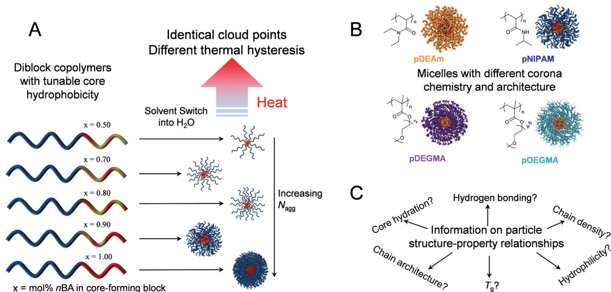
Scheme 1 A: Schematic of one series of diblock copolymers with identical corona-forming blocks and tunable p( n BA- co -DMA) core compositions that self-assemble in water to yield micelles with a tunable N_{agg} . The resulting particles show identical cloud points but different thermal hysteresis when heated in solution. B: Design of four micellar series with different corona-forming blocks with distinct chemistry and architecture, but whose cores contain the same p( n BA- co -DMA) compositions. In each case, the chemical structure of the corona block is shown. C: Studying the thermo-responsive behaviors of the four micellar series gives information on the structure–property relationships regarding thermal hysteresis in thermo-responsive self-assemblies.
