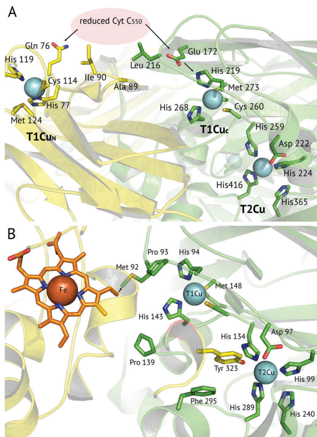
Fig. 6 Proposed electron transfer routes between the redox centres of 3-domain CuNiRs. In (A) HdNiR the external electron donor partner protein cyt. C550 is proposed to bind to a hydrophobic patch spanning the N-terminal (near Ala89, Ile90) and cupredoxin domains (near Leu216), where it is positioned for electron transfer to both the T1Cu N and T1Cu C sites (indicated by arrows). 74 In (B) RpNiR , the proposed internal electron transfer route is from the haem (CBC atom) to Met92 and to the T1Cu site. 75 Interface and T2Cu water molecules have been omitted from the figures for clarity.
