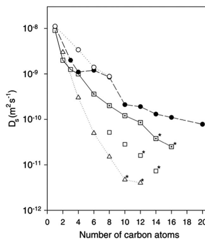
Fig. 2 Self-diffusivities obtained at 300 K from MD simulations ( \circ ), 35 hierarchical simulations ( \bullet ), 50 QENS in Na-ZSM-5 ( \square ), 46 QENS in silicalite-1 ( \square^* ) 47 and PFG-NMR ( \Delta ). 49 * = extrapolation to 300 K. Figure reproduced from ref. 47 with permission from the American Chemical Society.
