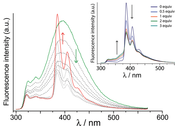
Fig. 3 Main figure: changes in fluorescence during addition of 3 to a solution of cage H ( 1 \mu\text{M} ) in water resulting in formation of H:3 : the cage fluorescence (green) is progressively quenched, and sensitised fluorescence from 3 (red) grows in. Inset: Restoration of fluorescence of cage H , and loss of sensitised pyrene fluorescence, on addition of cycloundecanone (3 equiv.) which displaces guest 3 from the cavity of H .
