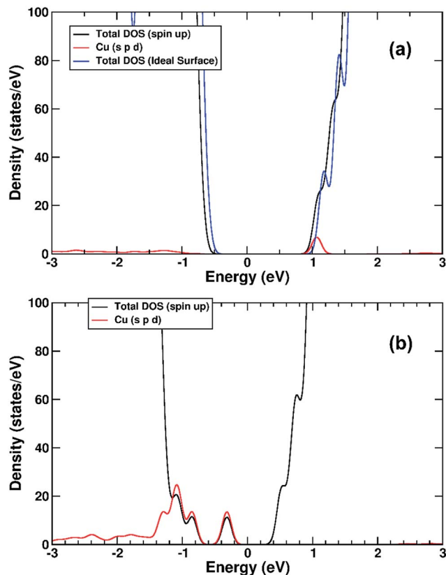
Fig. 10 (a) DOS of the \text{TiO}_2(R)\text{-Cu} system, spin-up channel only, aligned to the DOS of the ideal \text{TiO}_2(R) surface. (b) The spin up channel DOS of the final relaxed electron polaron system for the \text{TiO}_2(R)\text{-Cu} system. Cu contribution shown. The zero of the x-axis is fitted to the VBM for both plots.
