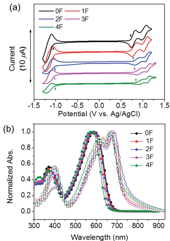
Fig. 1 (a) Cyclic voltammograms of 0F–4F dichloromethane solutions containing 0.1 \text{ mol L}^{-1} \text{ Bu}_4\text{NPF}_6 and a scan rate of 50 \text{ mV s}^{-1} . (b) UV-vis absorption spectra of 0–4F chloroform solutions (filled circles) and films (open circles).
