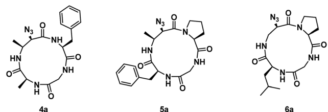
Fig. 2 Structures of azide ring-opened 13-membered \alpha_3\beta rings with varying side chains around the Azy residue.
