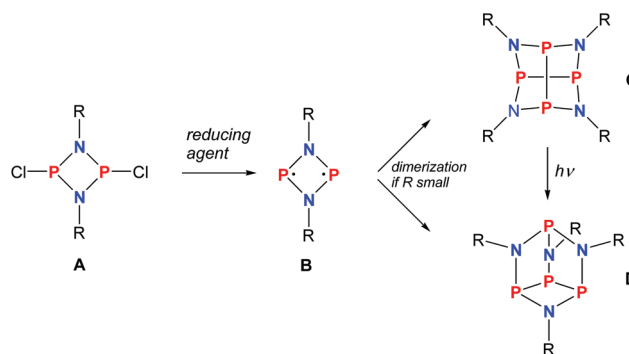
Fig. 1 Reduction of cyclodichlorodiphosphadiazane A yielding biradicaloid B or its dimers C and D depending on the steric strain.
