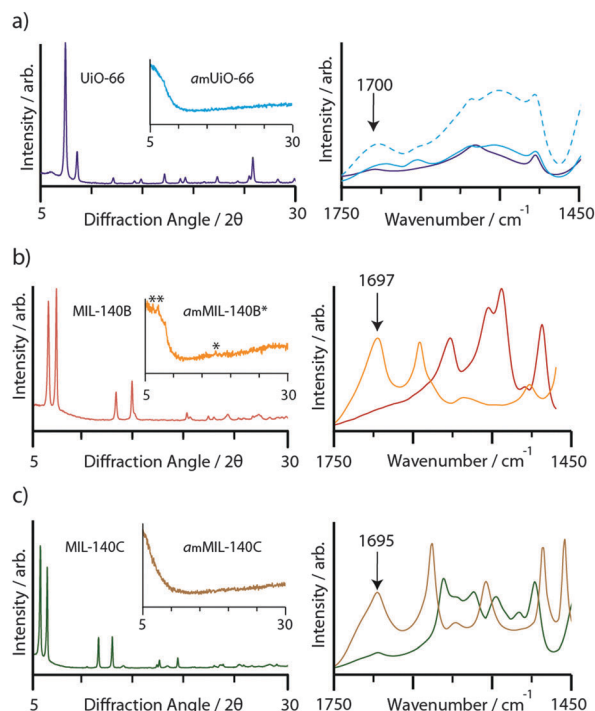
Fig. 2 \text{Cu K}\alpha_1 powder X-ray diffraction patterns, and IR spectra, of crystalline and (inset) amorphous samples (left hand plots), complete with IR spectra of the region 1450–1750 cm -1 (right hand plots). (a) UiO-66 : dark blue, a m UiO-66 : light blue, a m UiO-66 after 20 minutes ball milling: broken light blue, (b) MIL-140B : red, a m MIL-140B* : orange, (c) MIL-140C : green, a m MIL-140C : brown.
