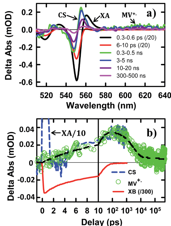
Fig. 3 TA spectra and kinetics of CdSe NS– MV^{2+} complexes measured with 400 nm excitation. (a) TA spectra evolution from 0.3 ps to 500 ns. The first two spectra have been reduced by a factor of 20 for better comparison. (b) Kinetics of MV^{2+} radical (green circles) and the complementary NS XB (red solid line) and XA/CS signal (blue dashed line). The latter have been scaled for better comparison. The black dashed line is a multi-exponential fit to the formation and decay kinetics of MV^{2+} radical signal.
