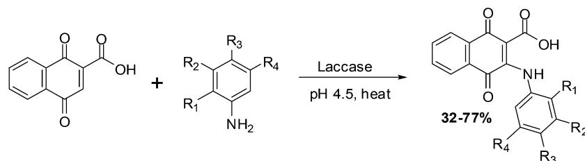
Scheme 2 Synthesis of aminonaphthoquinones 9–16.
