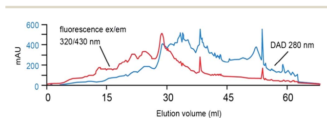
Fig. 6 HILIC-UV separation for Suwannee River DOM. Reproduced with permission from Woods et al. 133
