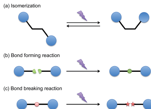
Fig. 1 Representative primary photochemical reactions; isomerization, bond forming and bond breaking reactions.
