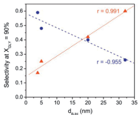
Fig. 14 Correlations between selectivities to dihydroxyacetone (DIHA – \blacktriangle ) and glyceric acid (GLYCEA – \bullet ) and the main pore size (calculated by the BJH method) for Au nanoparticles supported on mesoporous carbon supports. Reprinted with permission from ref. 144. Copyright 2012, Elsevier.
