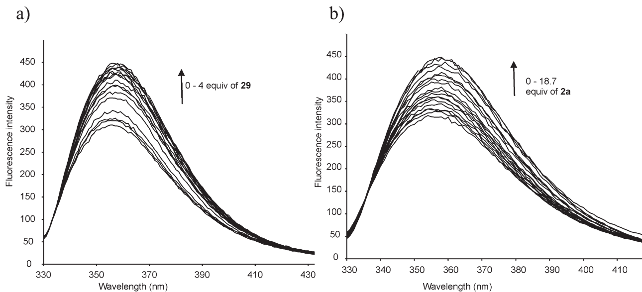
Fig. 7 Fluorescence titration of receptor 26 with \alpha -maltoside 29 (a) and \beta -glucopyranoside 2a (b) in \text{CHCl}_3 ; [ 26 ] = 8.51 \times 10^{-5} and 9.57 \times 10^{-5} M; Equiv. of 29 = 0.00–4.03; Equiv. of 2a = 0.00–18.69. Excitation wavelength 324 nm. Fluorescence intensity increased with increasing sugar concentration. 24
