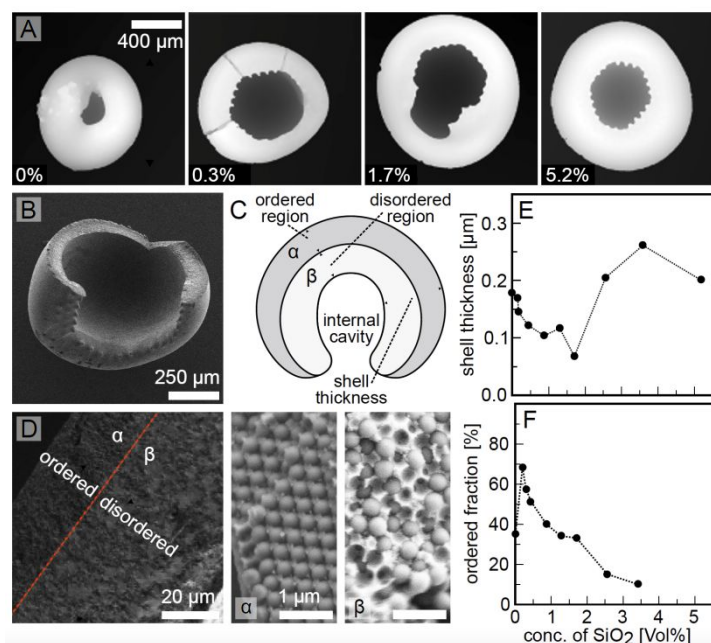
Fig. 4 Details of the supraparticle shell. (A) Topological rendering of a supraparticles bowl-side up for fixed PS (3.6 vol%) and varying SiO 2 volume fractions in the initial droplet, as indicated on each image. Confocal microscopy in reflection mode was used for imaging. (B) SEM micrograph of the final 3D morphology of a supraparticle resulting from a 3.6 Vol% PS + 1.7 Vol% SiO 2 droplet suspension. (C) Schematic illustrating the structural features of the supraparticles after complete evaporation. (D) SEM indicating the two different regions of the shell, with the dotted red line delineating the interface between them. The higher magnification SEM images show the closed-packed arrangement of the colloids in the outer part of the shell ( \alpha ) and a disordered arrangement in the inner region ( \beta ). (E) Shell thickness for increasing concentrations of silica in the deposited droplet at a constant PS concentration of 3.6 Vol%. (F) Percentage of the ordered shell region throughout the thickness of the shell for various concentrations of silica at a constant PS concentration of 3.6 Vol%.
