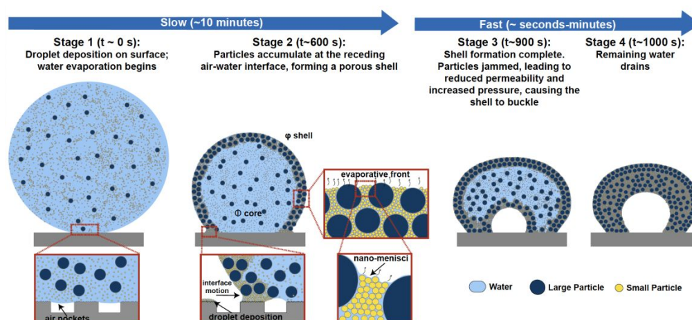
Fig. 2 Schematic illustrating the mechanism of supraparticle formation from the evaporation of a binary colloidal sessile droplet consisting of 2 species of particles with diameter ratio exceeding 10:1. Times t indicate approximate start times of each stage. The drawing is not to scale; in particular, the ratio of particle to droplet size is much smaller than pictured. The times included parenthetically correspond to the values obtained for 3 \mu\text{L} binary droplets consisting of 3.6 vol% PS and 1.7 vol% \text{SiO}_2 at ambient conditions (room temperature and pressure, and a relative humidity of \sim 20\% ).
