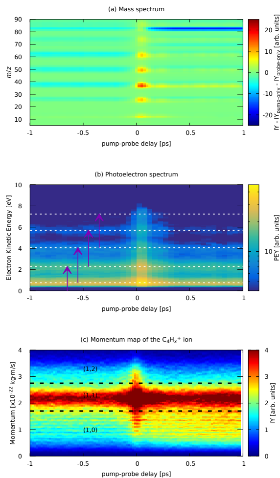
Fig. 7 Experimental parts of the pump (810 nm) – probe (405 nm) dependent MS (a) and photoelectron spectrum (b) of FLU, and (c) ion momentum distribution map of the C_4H_x^+ fragment. Horizontal lines in (b) indicate the positions of the ATI peaks from Figure 3. Purple arrows in (b) indicate the probe photon conversion of the ATI electrons. Horizontal lines in (c) show the approximate delimiters of the (1,0), (1,1), and (1,2) channels of the C_4H_x^+ ion. The ion yield (IY) in the MS corresponds to background-subtracted values, i.e., with corresponding values of pump-only and probe-only spectra subtracted. The full m/z -range version of (a) is available in the ESI.
