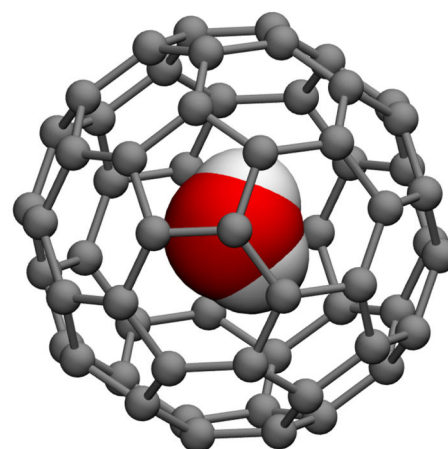
Fig. 5 Schematic depiction of the molecular structure of H 2 O@C 60 . Reproduced from ref. 40, with the permission of AIP Publishing.
