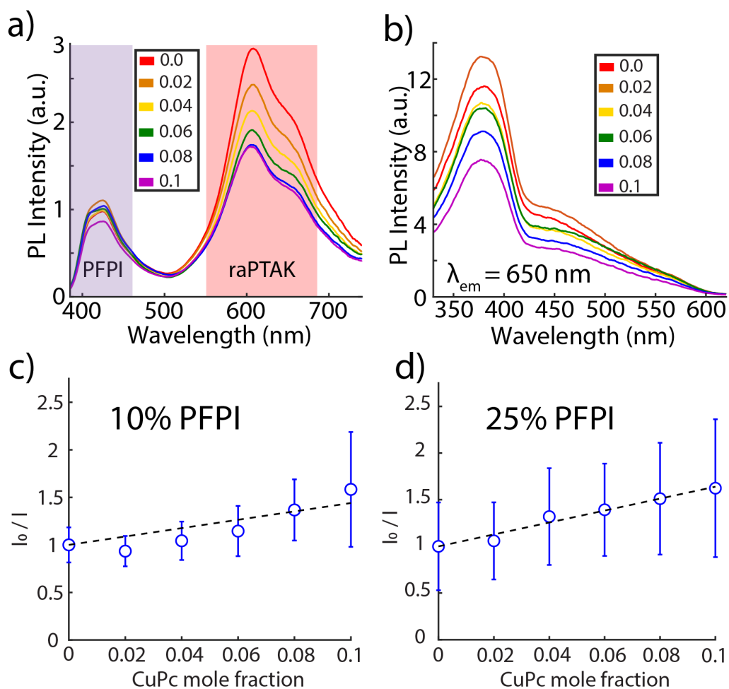
Figure 10. (a) PL spectra of PFPI/raPTAK/oCuPc:DOTAP complexes as a function of oCuPc mole fraction. (b) PLE spectra of the same complexes with the PL wavelength fixed at 650 nm, corresponding to raPTAK emission. Samples in (a) and (b) contained 25% PFPI relative to raPTAK (50% relative to DOTAP). Similar results are shown for 10% PFPI in the Supporting Information (Figure S8). (c) Stern-Volmer plot of raPTAK PL as a function of oCuPc mole fraction for 10% PFPI relative to raPTAK. (d) same as (c) but for 25% PFPI. PL integration windows are indicated by colored bars in (a).
