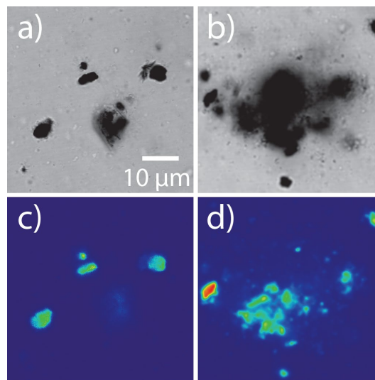
Figure 7. Transmission (top row) and PL (bottom row) images of raPTAK/oCuPc:DOTAP samples prepared at RT and 70°C (a/c and b/d respectively). The oCuPc loading was 5%.
