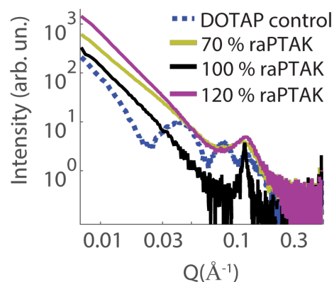
Figure 6. SAXS intensities of raPTAK/liposome complexes as a function of raPTAK % relative to lipids prepared at room temperature. The dashed blue line shows the pure DOTAP liposome control, whereas solid lines correspond to various raPTAK coverages in raPTAK/liposome complexes.
