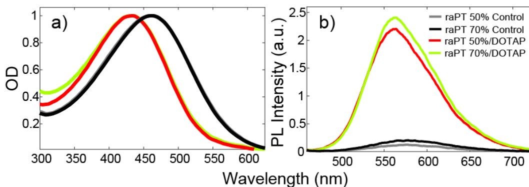
Figure 5. Steady-state photophysics of raPTAK/ DOTAP liposome complexes. (a) OD and (b) PL spectra normalized by OD at \lambda_{\text{max}} . The percentage in the legend refers to raPTAK ionic charges relative to those of the lipids. Controls are isolated pristine raPTAK solutions. Binding to DOTAP liposomes leads to a blue shift in raPTAK OD and a concomitant increase in its PL intensity relative to control samples.
