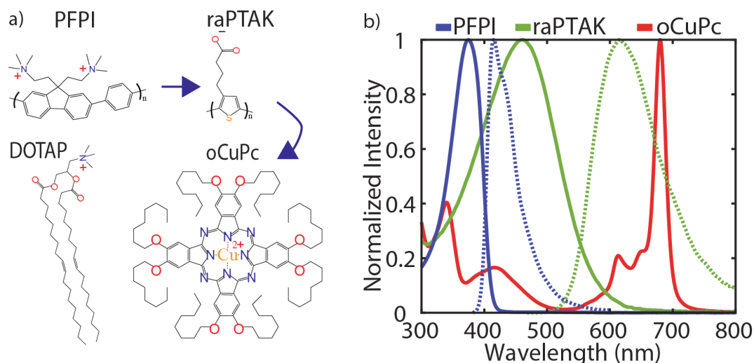
Figure 2. (a) Chemical structures of anionic CPE raPTAK, cationic CPE PFPI, cationic lipid DOTAP, and neutral phthalocyanine derivative oCuPc. (b) Peak-normalized optical density (solid) and photoluminescence (dashed) for the organic semiconductors shown in (a). Blue arrows show the path of exciton flow.
