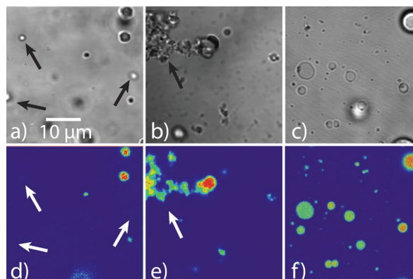
Figure 4. Transmission (top row) and PL (bottom row) images of raPTAK/DOTAP samples prepared at RT, 35°C, and 70°C (a/d, b/e, c/f respectively). The PL image color temperature is proportional to the relative PL intensity within a given image.
