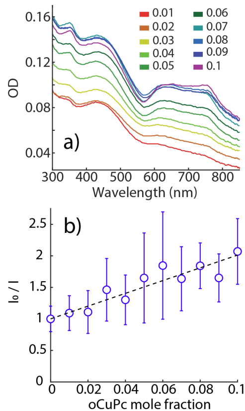
Figure 8. (a) OD of raPTAK/oCuPc:DOTAP liposome complexes as a function of oCuPc mole fraction relative to lipids. (b) Stern-Volmer plot of integrated raPTAK PL, which shows progressive quenching of raPTAK PL with increasing [oCuPc].
