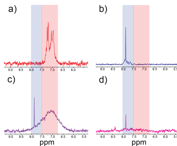
Figure 9. ^1\text{H} NMR spectra of (a) isolated raPTAK solution, (b) isolated PFPI solution, (c) PFPI/raPTAK complex solution, and (d) PFPI/raPTAK/liposome complex solution.
