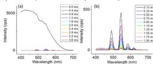
Figure 2. TRES of Tb@bGQDs excited at 330 nm showing spectra recorded (a) 0-3.6 ms and (b) 0.15-1.95 ms after excitation.
