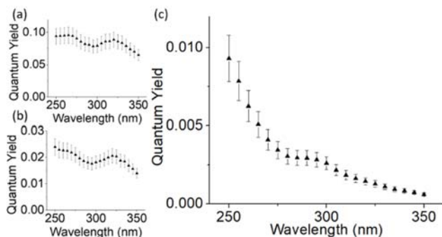
Figure 4. Quantum yield at varying excitation wavelengths (a) bGQD, (b) the bGQD peak from Tb@bGQD, and (c) the Tb 3+ peaks from Tb@bGQD.
