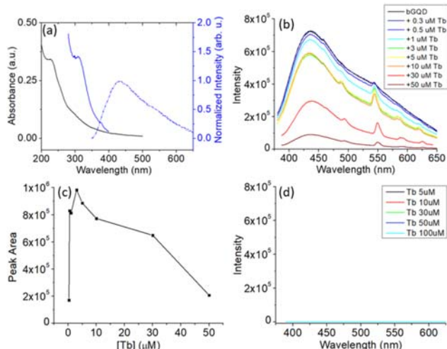
Figure 1. (a) Absorption (black), excitation (solid blue) and emission (dashed blue) spectra of bGQDs (5 µg/mL) in water excited at 330 nm. (b) Emission spectra of TbCl 3 titration into aqueous solution of bGQDs. (c) Plot of emission intensity recorded at 545 nm from (b) the TbCl 3 titration. (d) Photoluminescence of TbCl 3 at varying concentrations in water excited at 330 nm.
