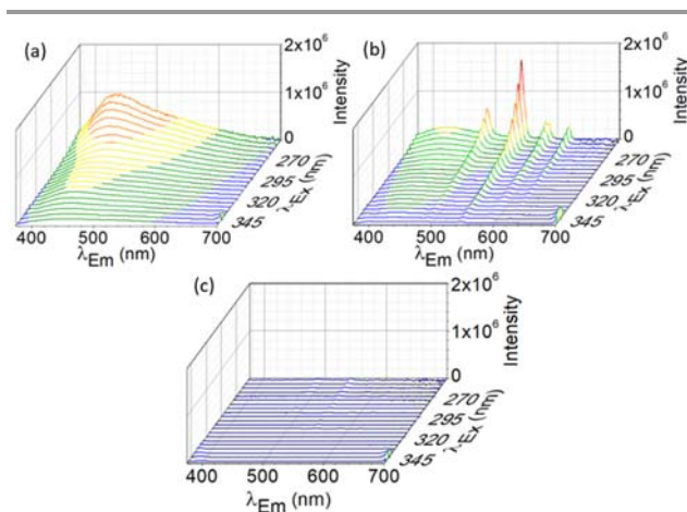
Figure 3. 3D emission spectra of (a) bGQD (10 \mu g/mL) (b) Tb@bGQD (10 \mu g/mL and 6 \mu M) and (c) TbCl 3 (6 \mu M).
