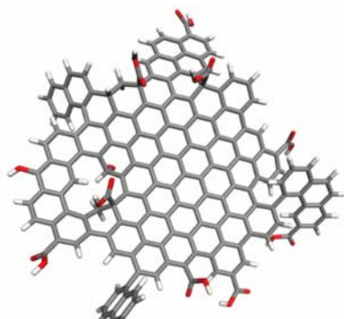
Figure 5. Schematic showing sp^2 carbon core with oxidative defects. Small organic molecule-like moieties on the periphery could partake in binding and sensitizing Tb^{3+} .
