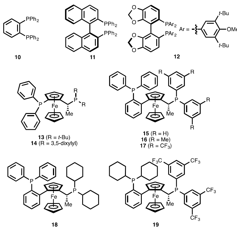
Figure 1: Ligands Examined in the CuH-catalyzed Conjugate Reduction of Ynenoate 8aa .
