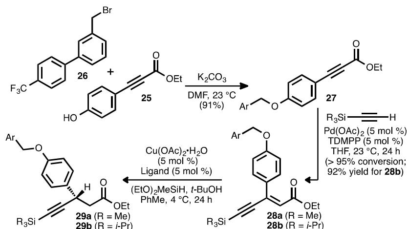
Scheme 5: Synthesis of β-Alkynyl Esters 29a and 29b en route to AMG 837 (24).
