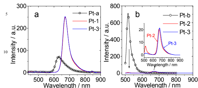
Fig. 5 Emission of the complexes to demonstrate intramolecular singlet energy transfer. (a) Pt-a ( c = 2.0 \times 10^{-5} M), Pt-1 ( c = 0.5 \times 10^{-5} M) and Pt-3 ( c = 1.0 \times 10^{-5} M), \lambda_{\text{ex}} = 424 nm. (b) Pt-b ( c = 1.0 \times 10^{-5} M), Pt-2 ( c = 0.3 \times 10^{-5} M) and Pt-3 ( c = 1.0 \times 10^{-5} M), \lambda_{\text{ex}} = 490 nm. In (a) or (b), optically matched solutions at the excitation wavelength were used therefore the concentration are different. In deaerated toluene, 20 °C.
