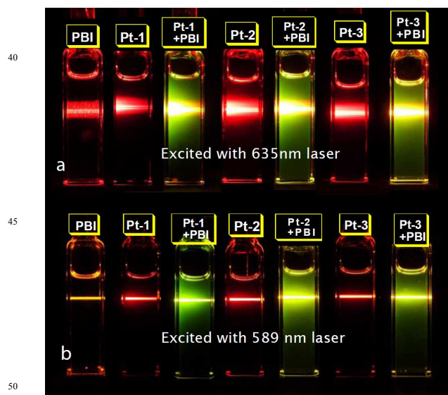
Fig. 13 Photographs of the TTA upconversion. Emission of triplet photosensitizer alone and the TTA upconversion. Excited with a continuous 635 nm laser (10 mW). c[\text{complexes}] = 1.0 \times 10^{-5} \text{ M} . For Pt-1 , c[\text{PBI}] = 2.6 \times 10^{-5} \text{ M} ; for Pt-2 , c[\text{PBI}] = 4.0 \times 10^{-5} \text{ M} . In deaerated toluene. 20 °C.
