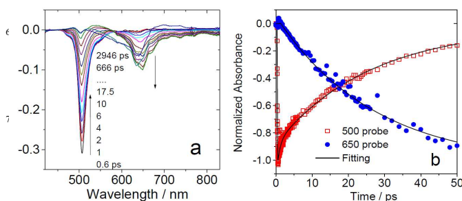
Fig. 8 Picosecond ultrafast transient absorption spectra of Pt-2 upon femtosecond pulsed laser excitation at 504 nm. (a) Transient absorption spectra after pulsed laser excitation at 504 nm. (b) Decay traces at 500 nm and 650 nm. c = 1.0 \times 10^{-5} M in toluene at 20 °C.
