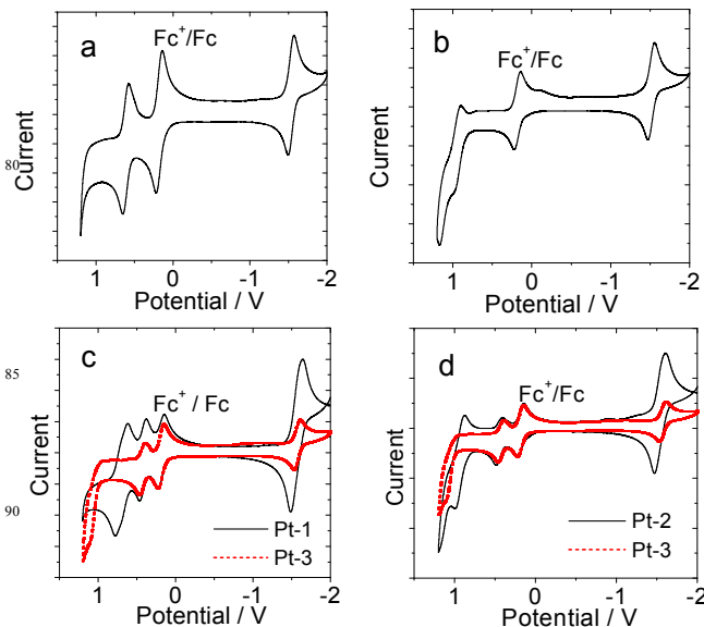
Fig. 2 Cyclic voltammogram of the complexes. (a) Pt-a , (b) Pt-b , (c) Pt-1 , (d) Pt-2 . The data of Pt-3 was presented in (c) and (d) for comparison. Ferrocene (Fc) was used as internal reference ( E_{1/2} = +0.64 V (Fc + /Fc) vs. standard hydrogen electrode). In deaerated CH 2 Cl 2 containing 0.5 mM photosensitizers with ferrocene, 0.10 M Bu 4 NPF 6 as supporting electrolyte, Ag/AgNO 3 reference electrode. Scan rates: 100 mV/s. 20 °C.
