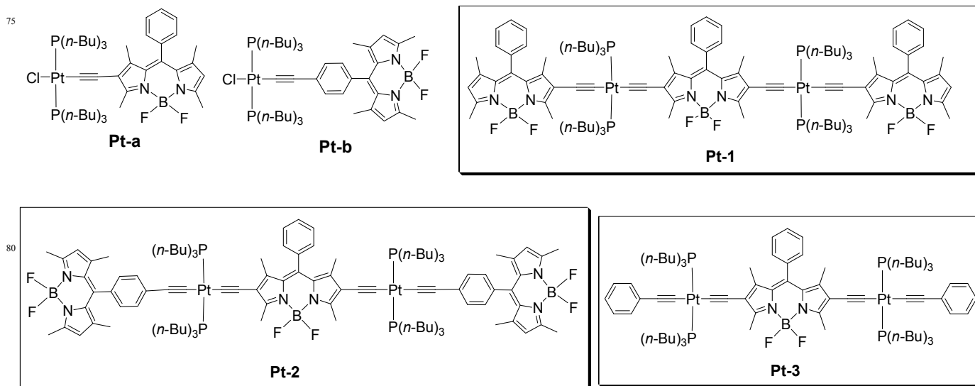
Scheme 1. Pt(II) complexes used in the study. The known complex Pt-3 is also presented.
