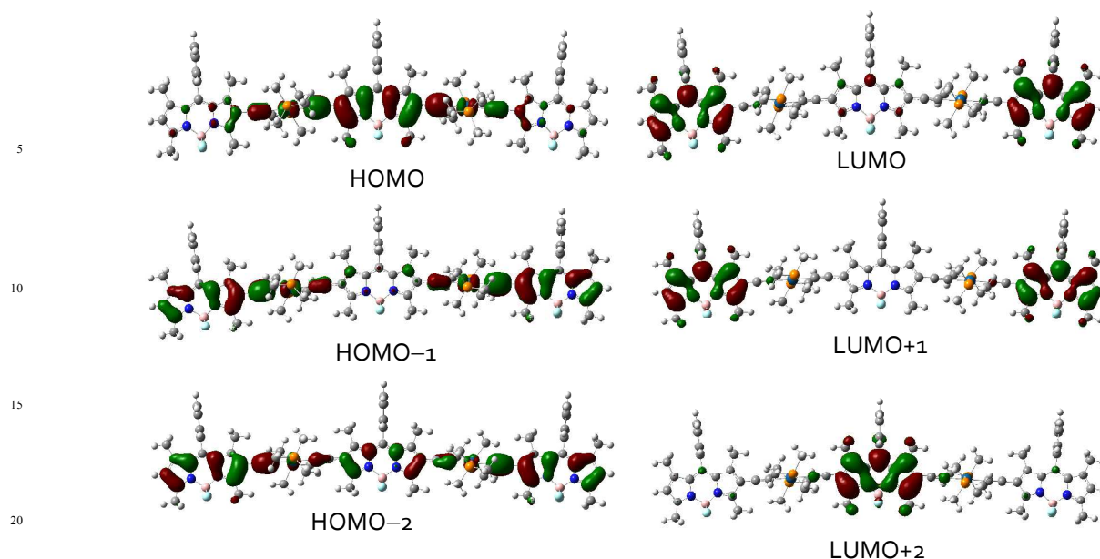
Fig. 10 Electron density maps of the frontier molecular orbitals of complex Pt-1 based on the optimized ground state geometry. The solvent toluene was considered in the calculations (PCM model). Calculated at the B3LYP/GENCP/LANL2DZ level with Gaussian 09W.
