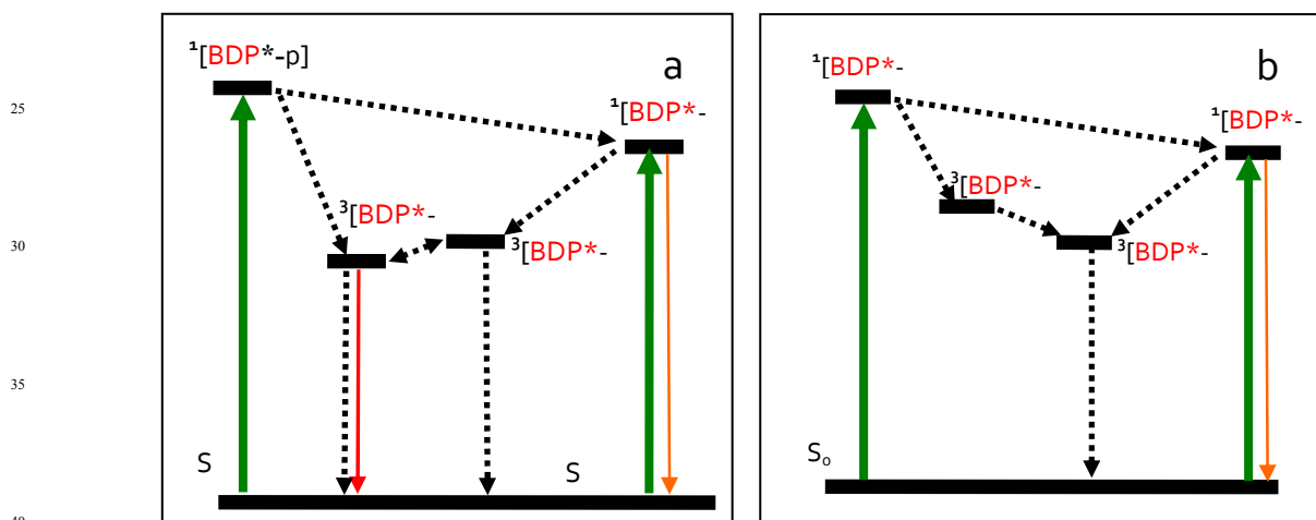
Scheme 3. Qualitative Energy Level Diagram of complexes (a) Pt-1 and (b) Pt-2 . BDP stands for Bodipy. BDP-c stands for the central coordination Bodipy part. BDP-p stands for the peripheral coordination Bodipy part.
