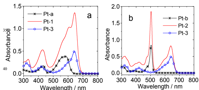
Fig. 3 UV-Vis absorption spectra of the complexes. (a) Pt-a , Pt-1 and Pt-3 . (b) Pt-b , Pt-2 and Pt-3 . c = 1.0 \times 10^{-5} M in toluene, 20 °C.
