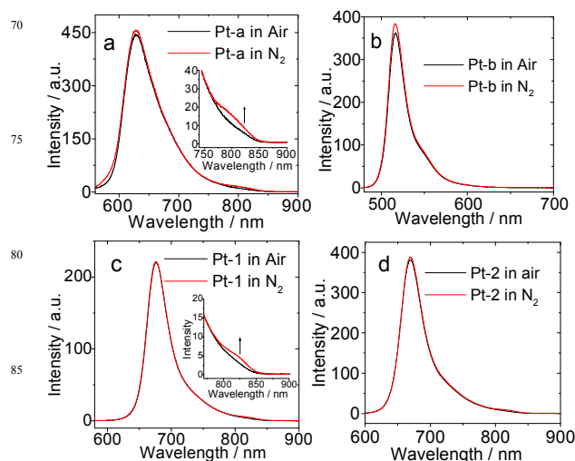
Fig. 4 Emission of the complexes under N 2 and air atmosphere. (a) Pt-a ( \lambda_{\text{ex}} = 550 nm), (b) Pt-b ( \lambda_{\text{ex}} = 470 nm), (c) Pt-1 ( \lambda_{\text{ex}} = 570 nm), (d) Pt-2 ( \lambda_{\text{ex}} = 590 nm). c = 1.0 \times 10^{-5} M in aerated or deaerated toluene at 20 °C.
