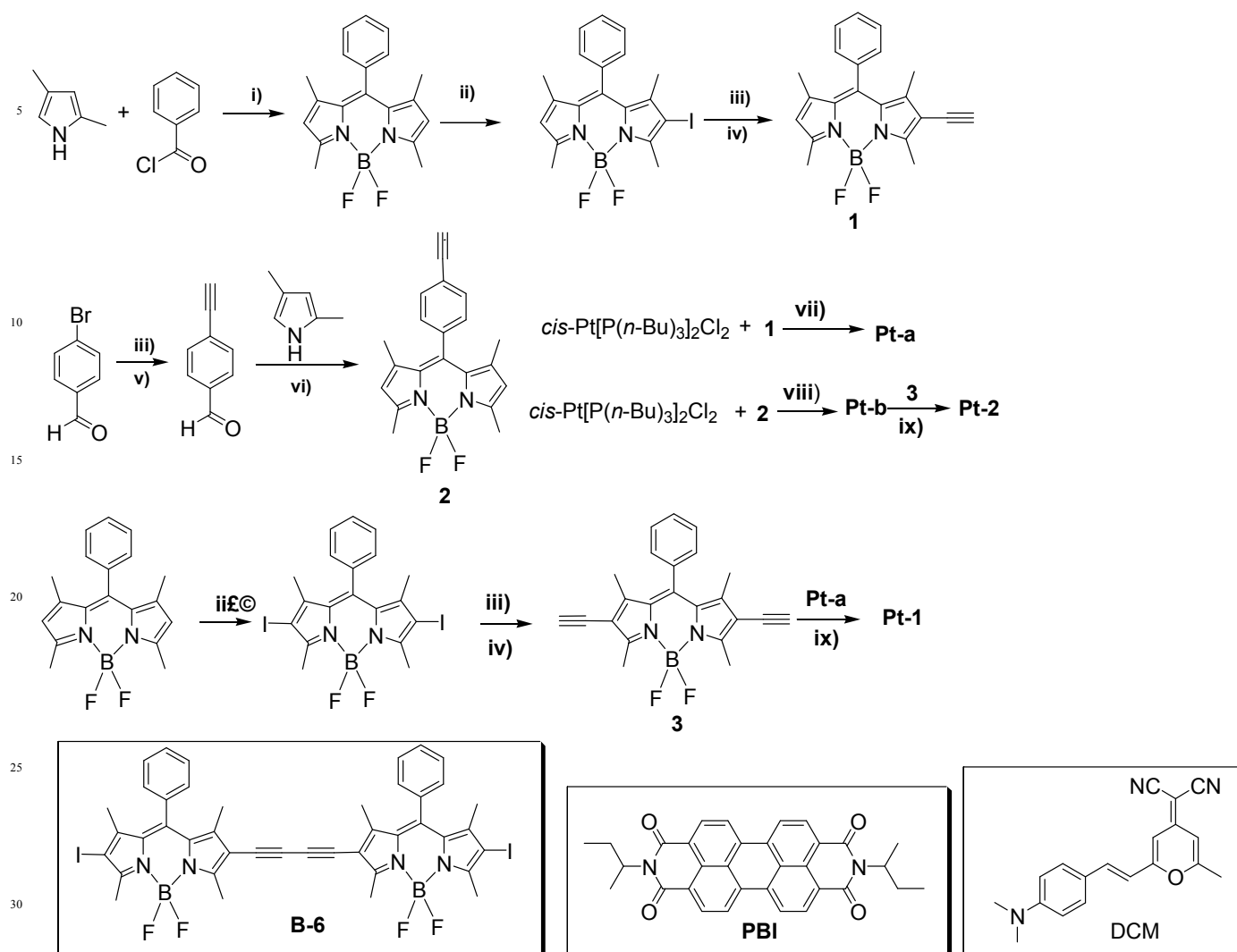
Scheme 2. Preparation of the ligands and the Pt(II) complexes. The model complex Pt-3 , triplet acceptor PBI used in TTA upconversion and the standards ( B-6 , DCM ) for determination of the fluorescence quantum yields are also presented. Reagents and conditions: (i) dry \text{CH}_2\text{Cl}_2 , \text{BF}_3\cdot\text{OEt}_2 , \text{NEt}_3 ; (ii) NIS, RT; (iii) trimethylsilylacetylene, \text{Pd}(\text{PPh}_3)_2\text{Cl}_2 , \text{PPh}_3 , \text{CuI} , \text{NEt}_3 , reflux, 8 h; (iv) \text{Bu}_4\text{NF} , THF, -78^\circ\text{C} ; (v) \text{K}_2\text{CO}_3 , MeOH, RT, 3 h; (vi) dry \text{CH}_2\text{Cl}_2 , \text{CF}_3\text{COOH} , \text{BF}_3\cdot\text{OEt}_2 , \text{NEt}_3 ; (vii) distilled THF, \text{NH}_4\text{Et} , \text{CuI} , -78^\circ\text{C} to RT, 8 h; (viii) \text{NH}_4\text{Et} , 45^\circ\text{C} , 8 h; (ix) THF/ \text{HNEt}_2 , \text{CuI} , 0-5^\circ\text{C} .
