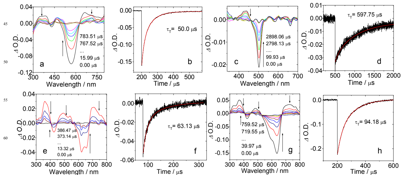
Fig. 7 Nanosecond time-resolved transient difference absorption spectra and the decay curves of the Pt(II) complexes. (a) complex Pt-a , (b) decay of Pt-a at 584 nm; (c) Pt-b , (d) decay of Pt-b at 504 nm ( \lambda_{\text{ex}} = 503 nm pulsed laser); (e) Pt-1 , (f) decay curve of Pt-1 at 644 nm; (g) Pt-2 , (h) decay curve of Pt-2 at 640 nm. With nanosecond pulsed laser excitation ( \lambda_{\text{ex}} = 532 nm). c = 1.0 \times 10^{-5} M in deaerated toluene at 20 °C.
