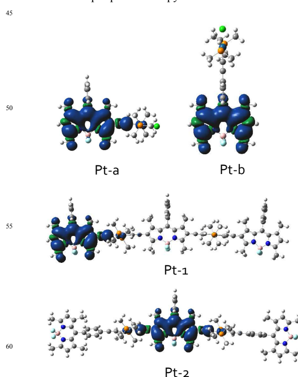
Fig. 9 Isosurfaces of spin density of the complexes Pt-a , Pt-b , Pt-1 and Pt-2 . Calculated at the optimized triplet state geometries. Toluene was used as solvent in the calculations (PCM model). Calculation was performed at B3LYP/GENECP/ LANL2DZ level with Gaussian 09W.
