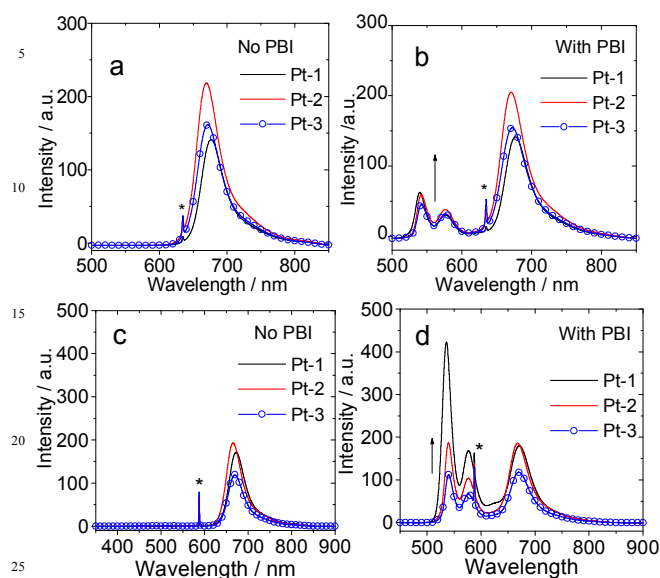
Fig. 12 Upconversions with Pt-1 , Pt-2 and Pt-3 as the triplet photosensitizers and PBI as triplet acceptor. (a) Photoluminescence spectra of the photosensitizers alone at 635 nm excitation (10 mW). (b) Photoluminescence spectra in the presence of PBI . Excited with a 635 nm laser (10 mW). (c) Photoluminescence spectra of the photosensitizers alone at 589 nm excitation (5 mW). (d) Photoluminescence spectra of the complexes in presence of PBI . Excited with a 589 nm laser (5 mW). For Pt-1 , c[\text{PBI}] = 2.6 \times 10^{-5} \text{ M} ; for Pt-2 , c[\text{PBI}] = 4.0 \times 10^{-5} \text{ M} ; for Pt-3 , c[\text{PBI}] = 4.1 \times 10^{-5} \text{ M} . The asterisks indicated the scattered laser (589 nm and 635 nm). c[\text{photosensitizers}] = 1.0 \times 10^{-5} \text{ M} in deaerated toluene at 20 °C.
