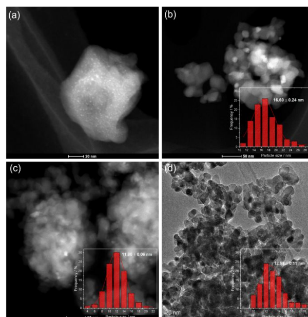
Fig. 1 HAADF-HRTEM images of (a) 1 wt% Pd/SSZ-13, (b) 1 wt% Pd/ \text{TiO}_2 , (c) 1 wt% Pd/ \text{MnTiO}_2 , and (d) 1 wt% Pd/ \text{ZrO}_2 catalysts and Pd particle size distributions on Pd/metal oxide catalysts.
