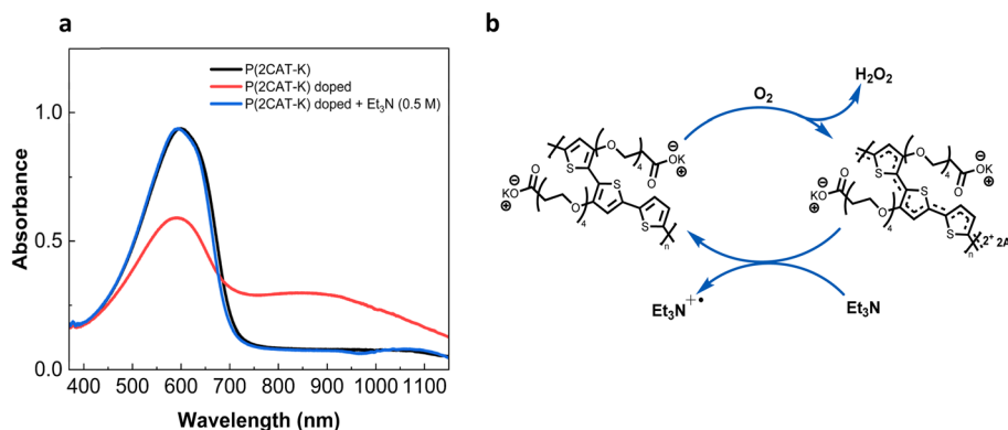
Fig. 3 (a) UV-Vis absorption spectra of a freshly prepared polymer aqueous nanodispersion (black line) sparged with O 2 (red line) and then mixed with 0.5 M of Et 3 N (blue line). The disappearance of the polaron peak and the recovery of the \pi - \pi^* transition peak shows the reversibility of the polymer oxidation by addition of the Et 3 N reducing agent. (b) Scheme of the polymer doping/dedoping cycle. P(2CAT-K) reduces O 2 to H 2 O 2 and then it is regenerated by oxidizing Et 3 N to Et 3 N + .
