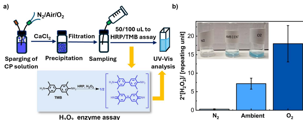
Fig. 2 (a) Scheme of the experimental procedure used for the autonomous production and quantification of H 2 O 2 by P(2CAT-K); (b) oxidation level of P(2CAT-K) based on measured H 2 O 2 concentration (multiplied by two) per number of polymer repeating unit obtained after exposing the same P(2CAT-K) aqueous nanodispersion to three different environments: O 2 , ambient air and N 2 atmosphere. Inset: Color of the filtrated solutions after addition to the HRP/TMB assay. The blue color is related to the charge-transfer complex formed by TMB in the presence of HRP enzyme and H 2 O 2 .
