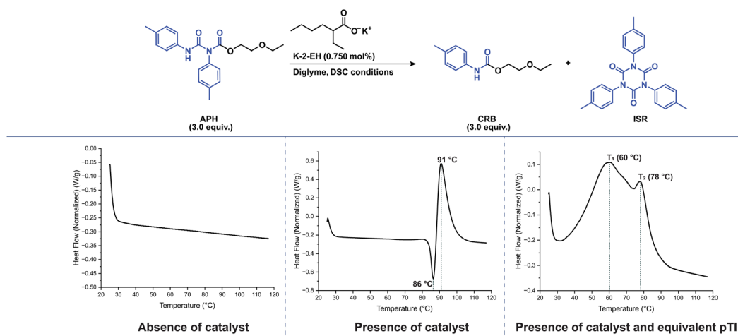
Fig. 3 DSC scans of APH catalytic degradation under three conditions: (i) in the absence of catalyst, (ii) in the presence of K-2-EH, and (iii) in the presence of K-2-EH with an equimolar amount of p TI. Catalytic reaction conditions (ii): APH (20 mg, 56.1 \mu mol), K-2-EH (0.750 mol% relative to APH, 0.4 \mu mol, 76.7 \mu g), diglyme (20 \mu L). Absence of catalyst (i): No K-2-EH was used. Presence of catalyst and equivalent of p TI (iii): K-2-EH (1.125 mol% relative to APH or 0.375 mol% relative to NCO/NCO derived molecules, 0.6 \mu mol, 112.5 \mu g), p TI (7.5 mg). DSC conditions: Temperature range 25–120 ^{\circ} C, heating ramp: 10 ^{\circ} C min^{-1} .
