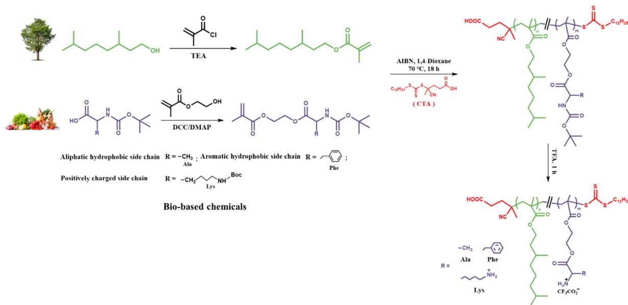
Fig. 1 Schematic diagram of the synthesis of bio-based monomers and amphiphilic random copolymers by RAFT polymerization.
