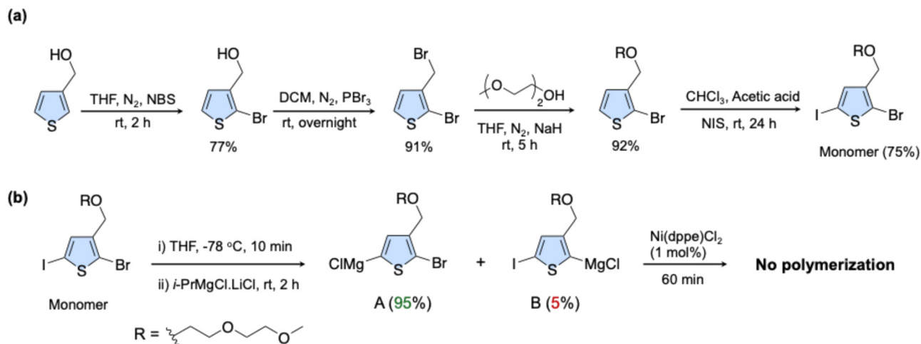
Scheme 1 (a) Synthesis, and (b) Grignard metathesis followed by polymerization of 2-bromo-5-iodo-3-((2-methoxyethoxy)methyl)thiophene.
