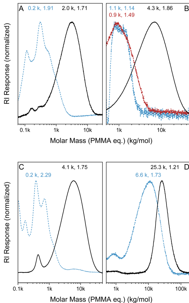
Fig. 7 SEC curves of intact polymers (black lines) and after degradation with ethylamine (1 M in THF, dashed blue lines) or NaOH (3.6 M in water, the dashed red line) for (A) p(\text{DMA}_{0.89}\text{-BOT}_{0.11})_n (Table 1 entry 5); (B) p(\text{DMA}_{0.84}\text{-BOT}_{0.16})_n (entry 6); (C) p(\text{DEVP}_{0.4}\text{-BOT}_{0.6})_n (entry 8); and (D) p(\text{Sty}_{0.98}\text{-BOT}_{0.02})_n (entry 9). The numbers indicate the estimated molar mass and dispersity, respectively. The estimated molar masses of the degraded fragments for (A) and (C) are imprecise as they are outside of the calibration range and appear to overlap with solvent signals.
