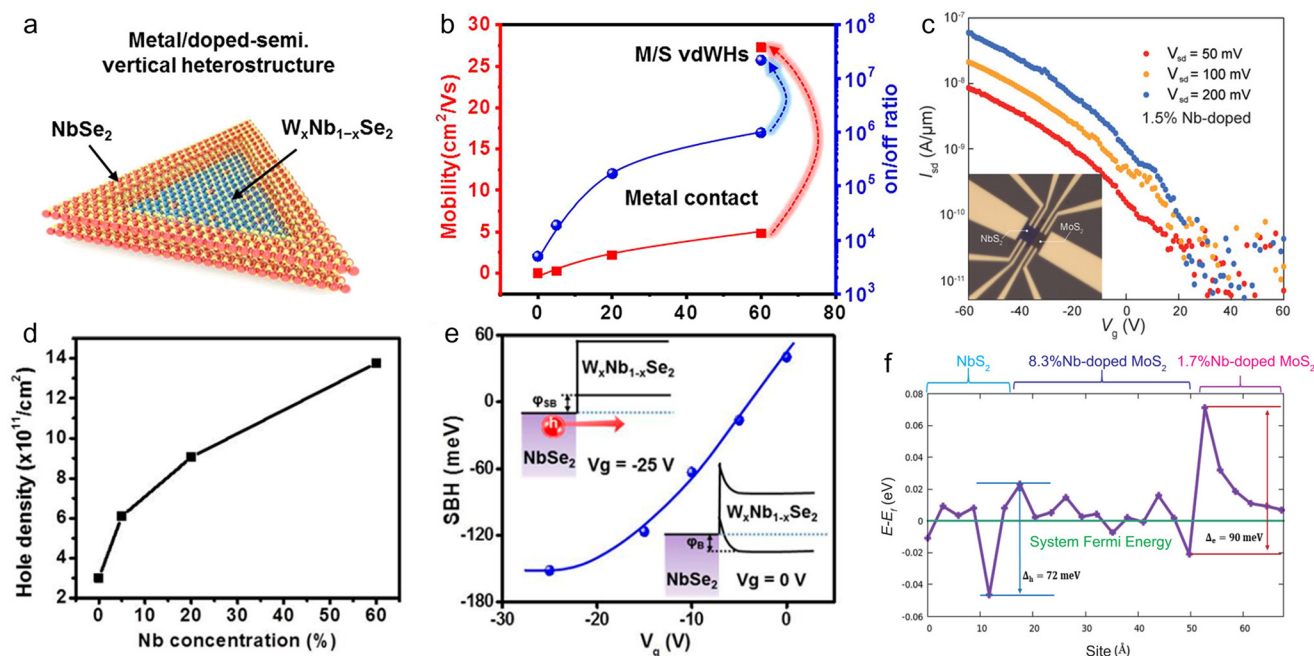
Fig. 8 Substitutional-doping-assisted ohmic contact engineering in 2D TMDs. (a) Schematic illustration of the \text{NbSe}_2/\text{W}_x\text{Nb}_{1-x}\text{Se}_2 metal/doped-semiconductor heterostructure synthesized by one-step CVD growth. (b) Comparison of field-effect mobility (left axis) and on/off ratio (right axis) between conventional metal-contacted \text{WSe}_2 and \text{NbSe}_2/\text{W}_x\text{Nb}_{1-x}\text{Se}_2 van der Waals heterostructures. (c) Transfer characteristics of the \text{NbS}_2 - \text{MoS}_2 lateral heterostructure, confirming stable p-type conduction. (Inset: OM image of the device). (d) Variation of hole carrier density in \text{WSe}_2 with increasing Nb incorporation (0–60%). (e) Extracted Schottky barrier height ( \Phi_{\text{SB}} ) as a function of gate voltage, showing a negative ( \Phi_{\text{SB}} ) ( \approx -0.68 eV) at the \text{NbSe}_2/\text{W}_x\text{Nb}_{1-x}\text{Se}_2 interface, indicative of p-type ohmic contact formation. (f) Calculated planar-averaged electrostatic potential across the \text{NbS}_2 - \text{MoS}_2 interface, revealing a minimal potential step ( \Delta E \approx 72 – 90 meV) that facilitates efficient hole transport. Reproduced from ref. 43 (panels a, b, d and e) and ref. 45 (panels c and f) under Creative Commons license (CC BY).
