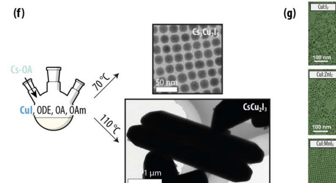
Fig. 12 Caesium copper halides as representative of copper halide SNCs. (a) Unit cell, copper cluster geometry, and simulated XRPD patterns of the most common compositions reported for Cs–Cu–X (where X = Cl, Br, I). (b) Absorption (dashed lines) and emission (solid lines) spectra of \text{Cs}_3\text{Cu}_2\text{I}_5 (blue) and \text{CsCu}_2\text{I}_3 (yellow), alongside a photo of the dispersion under UV excitation, and the corresponding photoluminescence decay curves. Adapted with permission from ref. 286, Copyright 2019, American Chemical Society. (c) The emission stems from a self-trapped exciton. (d) Representation of the Jahn–Teller distortion that occurs after excitation in \text{Cs}_3\text{Cu}_2\text{I}_5 . Adapted with permission from ref. 287, Copyright 2025, Springer. (e) Absorption and emission spectra, photoluminescence decay curves, and photo under UV excitation of a series of alloyed \text{Cs}_3\text{Cu}_2\text{X}_5 SNCs, alongside \text{CsCu}_2\text{Cl}_3 SNCs. Adapted with permission from ref. 288, Copyright 2020, American Chemical Society. (f) Scheme of the synthesis protocol for the synthesis of \text{Cs}_3\text{Cu}_2\text{I}_5 SNCs or \text{CsCu}_2\text{I}_3 microcrystals, alongside the TEM images of the respective materials. Adapted with permission from ref. 284, Copyright 2019, John Wiley and Sons. (g) TEM images of \text{Cs}_3\text{Cu}_2\text{I}_5 SNCs obtained using different halide additives, showing optimized morphology and narrow size distribution in the presence of \text{MnI}_2 . Adapted with permission from ref. 289, Copyright 2022, American Chemical Society. (h) TEM images of parent \text{Cs}_3\text{Cu}_2\text{Cl}_5 synthesized at 180 °C and used as sacrificial species for cation exchange with Zn, Bi, and Cd. The TEM images of the SNCs obtained from the cation exchange procedures are reported in the bottom row. Adapted with permission from ref. 290, Copyright 2023, American Chemical Society.
