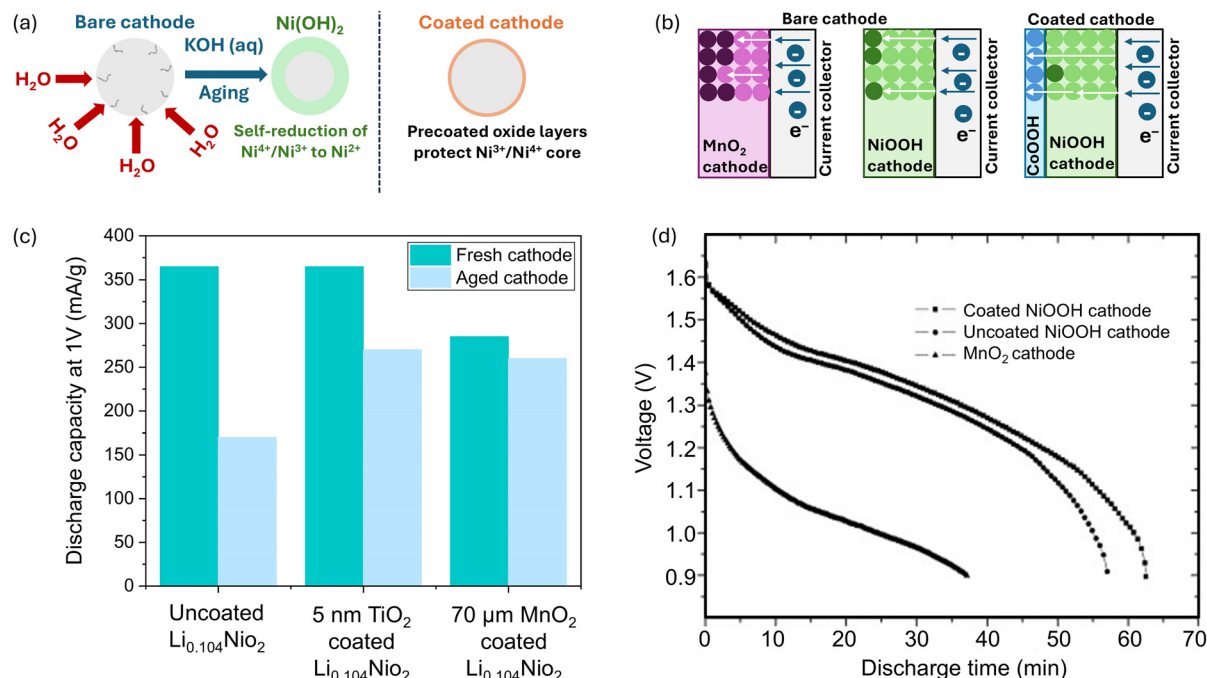
Fig. 9 Influence of surface coatings on the nanoscale phenomena occurring at the cathode-electrolyte interface and the electrochemical performance of the Ni cathodes with and without surface coatings. (a) Schematic illustration of the influence of surface coating on the stability of the cathode surface region in contact with the alkaline electrolyte. (b) Schematic depiction of electron conduction and discharge reaction occurring within the MnO 2 , NiOOH and coated NiOOH cathodes. (c) Bar chart of the specific discharge capacities of the uncoated, 5 nm TiO 2 - and 70 μm MnO 2 -coated Li 0.104 NiO 2 cathodes before (fresh) and after aging tests (aged). 122 (d) Discharge curves of the Zn-NiOOH battery with and without CoOOH surface coating of the cathode as well as the Zn-MnO 2 battery as a reference. Reproduced with permission from ref. 86. Copyright 2007, Elsevier.
