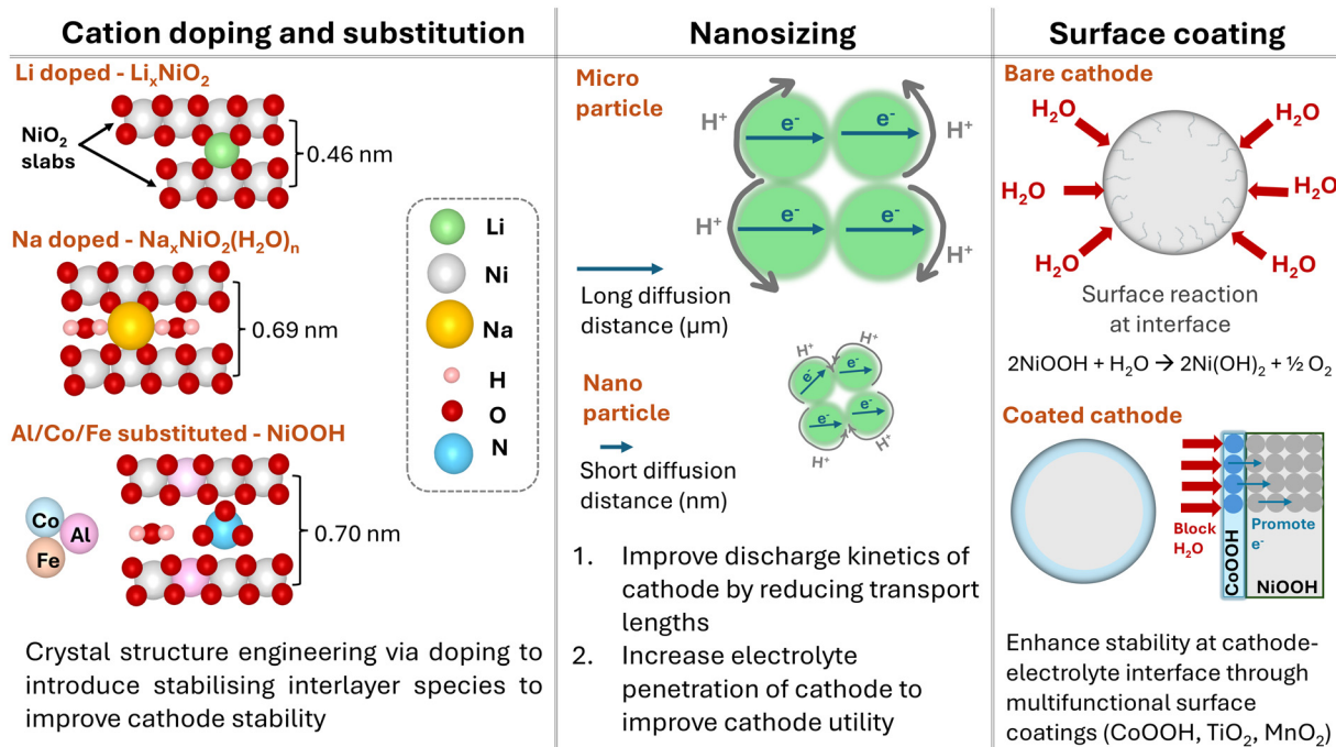
Fig. 12 Overview of the cathode design strategies and the accompanying nanoscale phenomena/features covered in this review.
