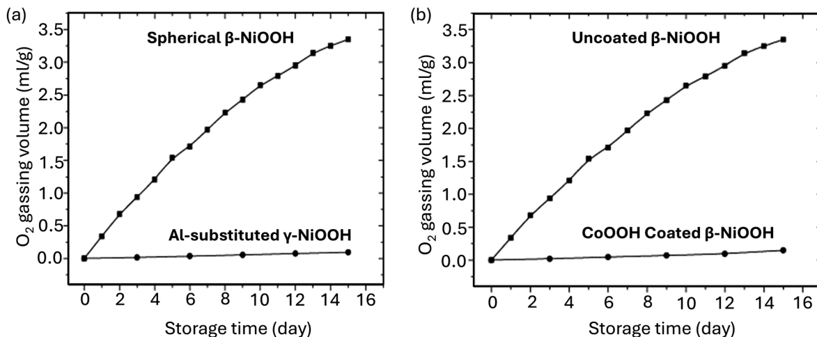
Fig. 10 O 2 evolution analyses of high-valent Ni cathodes after storage in a 9 M KOH solution at 60 °C, as a measure of the storage stability. (a) O 2 evolution measurement of the Al-substituted γ-NiOOH cathode. Reproduced with permission from ref. 115. Copyright 2007, Elsevier. (b) O 2 evolution measurement of the CoOOH-coated β-NiOOH cathodes. Reproduced with permission from ref. 86. Copyright 2007, Elsevier.
