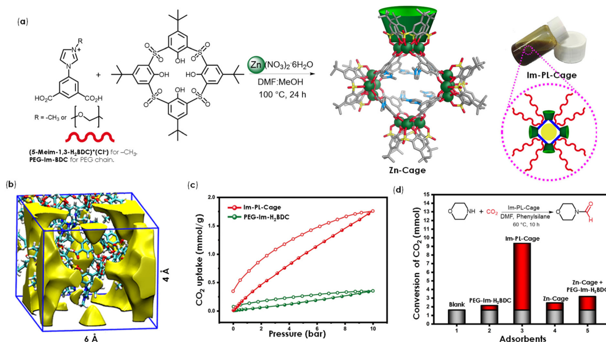
Fig. 3 (a) Schematic process of self-assembly to produce Zn-Cage and porous liquid Im-PL-Cage . (b) Snapshots of simulation boxes for Im-PL-Cage and pore space in Im-PL-Cage . (c) CO 2 adsorption–desorption isotherms of PEG-Im-H 2 BDC and Im-PL-Cage at ambient temperature. (d) The formylation reaction of morpholine with CO 2 and phenylsilane. Gray bars represent the transformed amount of CO 2 that was adsorbed on different adsorbents. Parts (b–d) adapted from ref. 55, https://doi.org/10.1038/s41467-023-39089-x . Copyright 2023, Springer Nature.
