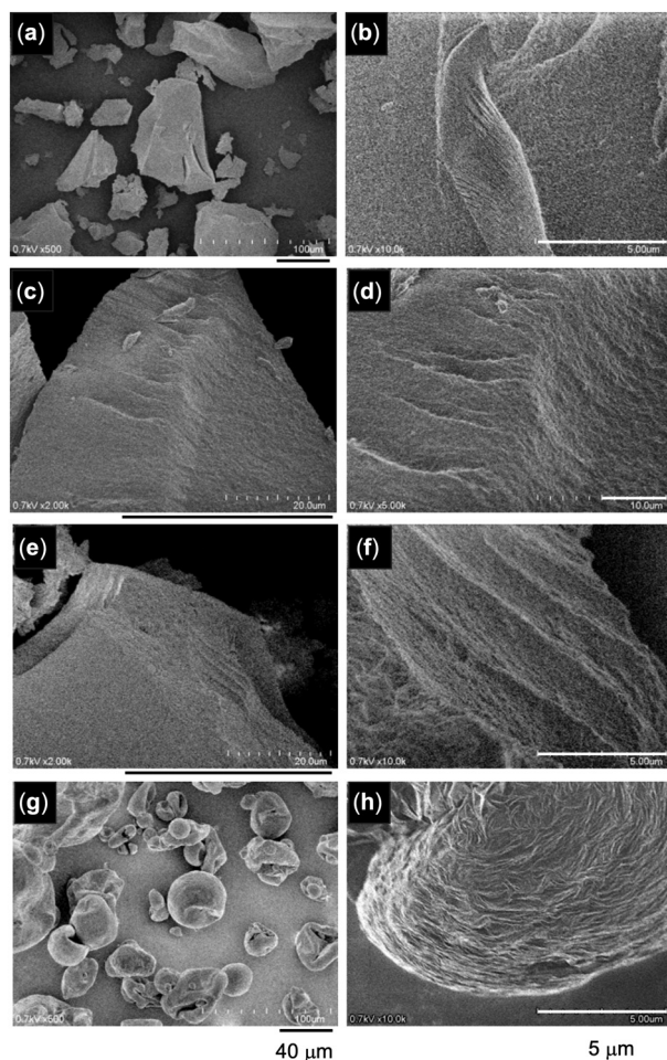
Fig. 9 FE-SEM images of (a and b) L-PAAm-DSBP composites, (c and d) M-PAAm-DSBP composites, (e and f) H-PAAm-DSBP composites and (g and h) DSBP. Black scale bars: 40 \mu\text{m} ; white scale bars: 5 \mu\text{m} .
