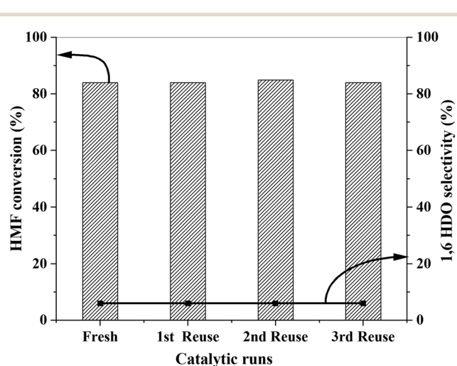
Fig. 5 Reusability of 5% PtRu/HAP catalyst. Reaction conditions: HMF: 1.59 mmol; HMF/Pt molar ratio: 155; methanol: 20 mL; H 2 : 2 MPa; temperature: 120°C; stirring: 1000 rpm; time: 2h.
