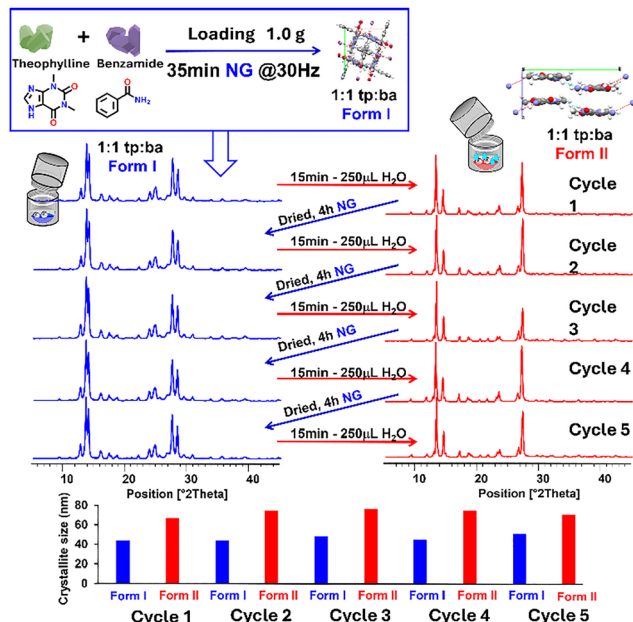
Fig. 37 Polymorph interconversion of 1:1 tp:ba cocrystals by ball milling at 1 g scale. Form I to Form II (LAG with 250 \mu L H 2 O, 15 min, 30 Hz). Form II is dried and reconverted to Form I (NG, 4 h, 30 Hz). Five turnover cycles performed. Crystallite sizes: Form I = \sim 40 nm; Form II = 60–80 nm. 10 Adapted from ref. 10 with permission from The Royal Society of Chemistry.
