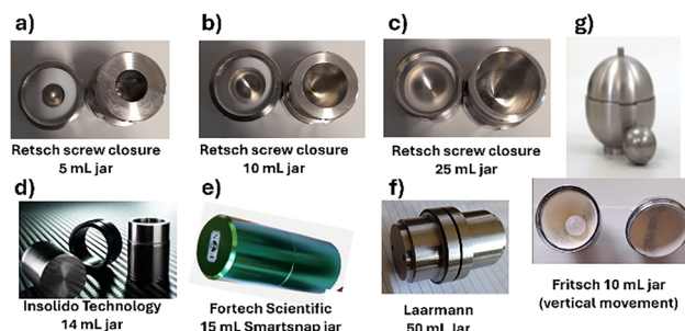
Fig. 3 Commercially available jars used for vibrational ball milling. The internal shape of the top and bottom caps are hemispheres, connected through a cylindric section. (a)–(f) Used under horizontal vibratory motion using ball mills depicted in Fig. 2(b). The milling jar in (g) is used for vertical motion using ball mills depicted in Fig. 2(c).
