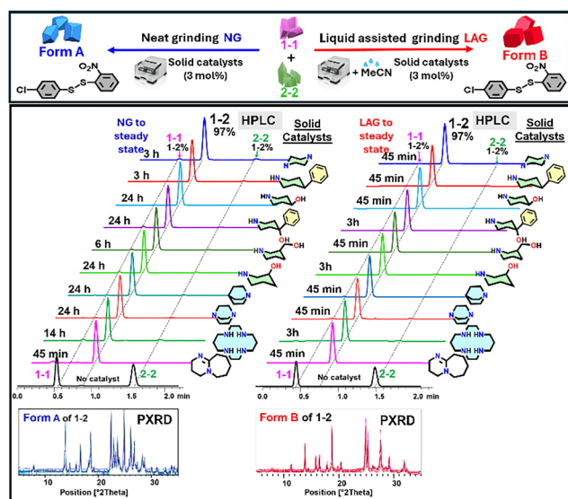
Fig. 18 Steady-state formation of 1-2 under NG and LAG conditions using 9 commercially available solid base catalysts and DBU. Top: Reaction scheme showing that NG produces Form A of 1-2 , while LAG with MeCN yields Form B of 1-2 . Left: NG reactions (3 mol% catalyst) milled to steady-state yields Form A to ~97 mol% with matching PXRD patterns below; right: LAG (MeCN) reactions with (3 mol% catalyst) milled to steady-state yields Form B to ~97 mol%. Despite consistent steady-state outcomes (Form A and Form B), the reaction kinetics vary significantly across base catalysts used specially under NG conditions. 54 Adapted with permission from ref. 54 [ChemSusChem, 2022, 15, e202102416]. Copyright [2022] Wiley-VCH GmbH.
