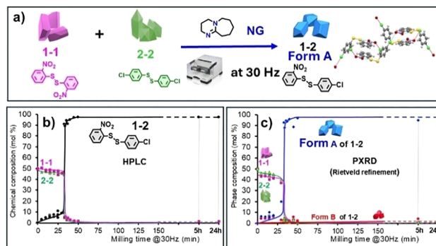
Fig. 11 Kinetic profiles prepared by HPLC and PXRD data for the disulfide 1-2 reaction under NG conditions. (a) Reaction scheme. (b) Kinetic profile from molecular composition (HPLC). (c) Kinetic profile from phase composition (PXRD, Rietveld). Each point of the kinetic profile represents an independent milling experiment. The total 1-2 content in (b) reflects the combined Form A and Form B contributions determined in (c). 51 Adapted from ref. 51 with permission from JACS, 2014, 136 , 16156–16166, Copyright (2014) American Chemical Society.
