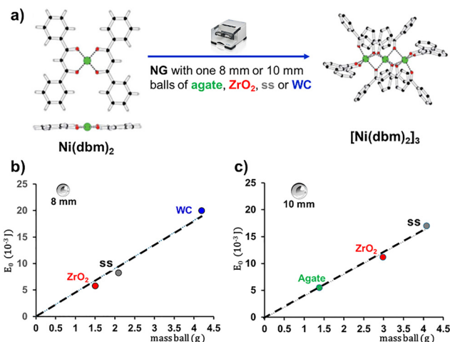
Fig. 58 Mechanochemical trimerization of brown \text{Ni}(\text{dbm})_2 \rightarrow green [\text{Ni}(\text{dbm})_2]_3 . (a) Reaction scheme. (b) and (c) Activation impact energy ( E_0 ) as a function of milling ball mass ( m_{\text{ball}} ). (b) 8 mm balls made from \text{ZrO}_2 , ss, and WC. (c) 10 mm balls made from agate, \text{ZrO}_2 , and ss. The fraction of reactant powder affected by critical loading conditions per unit time ( k_R ) correlates directly with E_0 . 74 Reproduced from ref. 74 with permission from [RSC], copyright [2022] and figures drawn with original data supplied by Maria Carta.
