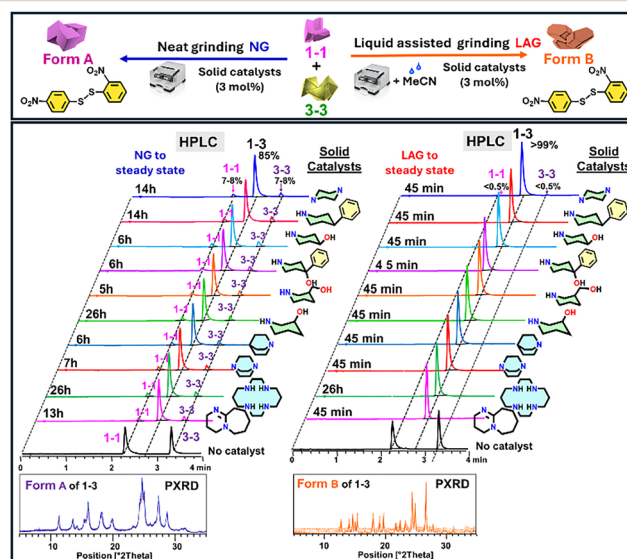
Fig. 19 Steady-state formation of 1-3 under NG and LAG conditions using solid base catalysts. Top: Reaction scheme showing that NG produces Form A of 1-3 , while LAG with MeCN yields Form B of 1-3 . Left: NG reactions (3 mol% catalyst) give ~85 mol% Form A of 1-3 , with the remaining 1-1 and 3-3 present at ~7–8 mol% each; with matching PXRD patterns below. Right: LAG reactions give >99 mol% Form B of 1-3 , with matching PXRD patterns below. Despite consistent steady-state outcomes (Form A vs. Form B), the reaction kinetics vary significantly across base catalysts used specially under NG conditions. 54 Adapted with permission from ref. 54 [ChemSusChem, 2022, 15, e202102416]. Copyright [2022] Wiley-VCH GmbH.
