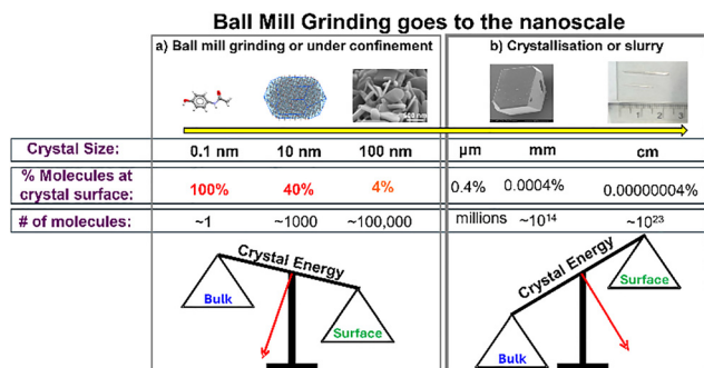
Fig. 28 Effect of crystal size on polymorph formation. (a) Ball milling produces nanocrystals with significant surface contributions; (b) solution or slurry crystallization generates \mu\text{m} – \text{cm} crystals where surface effects are negligible, so bulk stabilization dominates. Calculations by Aurora Cruz Cabeza.
