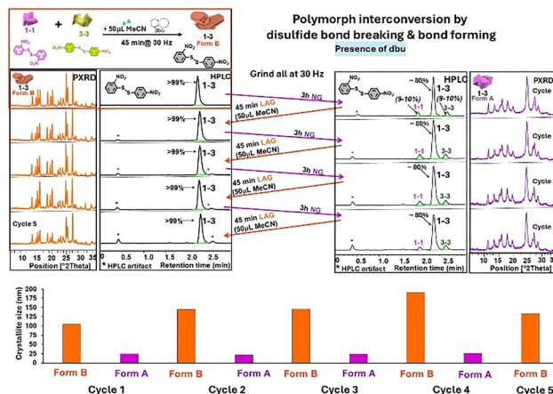
Fig. 33 Polymorph interconversion of 1-3 under NG and LAG milling. Initial Form B of 1-3 ( >99 mol% by HPLC) is dried and converted to Form A of 1-3 at \sim 80 mol% by NG (3 h, 30 Hz). Form A of 1-3 is reconverted to Form B of 1-3 at >99 mol% by LAG with 50 \mu L MeCN (45 min, 30 Hz). The cycle is repeated five times. Crystallite sizes: Form B of 1-3 = 110–180 nm; Form A of 1-3 = \sim 30 nm. 53 Adapted with permission from ref. 53. Copyright [2021] Wiley.
