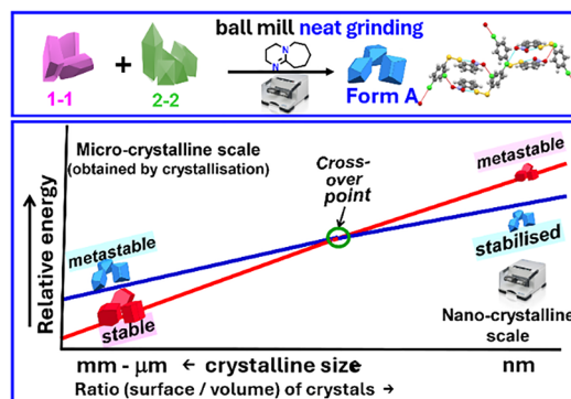
Fig. 29 Stabilization of Form A of 1-2 under NG ball-milling conditions. (a) Disulfide exchange scheme under NG conditions. (b) Nanosizing-induced stability crossover: Form B, stable at \mu\text{m} + sizes, becomes metastable at the nanoscale, while Form A, metastable at \mu\text{m} + sizes, becomes stable at the nanoscale. 51 Adapted from Navrotsky's work on iron oxyhydroxide. 58
