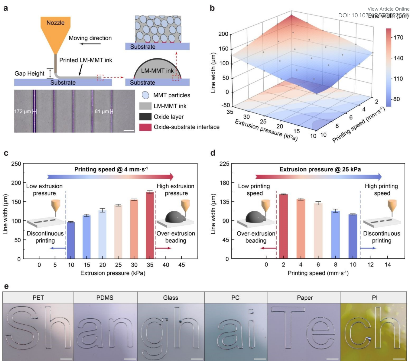
Figure 3 Direct ink writing of LM-MMT ink.
