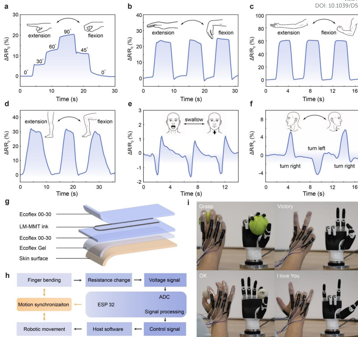
Figure 5 LM-MMT sensors for human motion monitoring and human-machine interaction.
