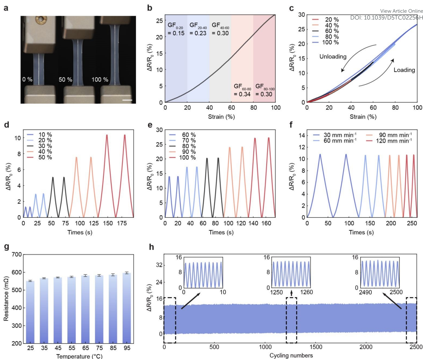
Figure 4 Mechanical and electrical performance of LM-MMT strain sensor.
