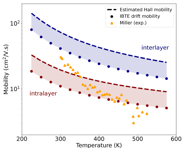
Fig. 3 IBTE hole drift mobility of SnO against temperature. Using a constant Hall factor of 1.77^{25} for the range of temperature, the approximate Hall mobility is also shown and compared with experimental results from ref. 64.
