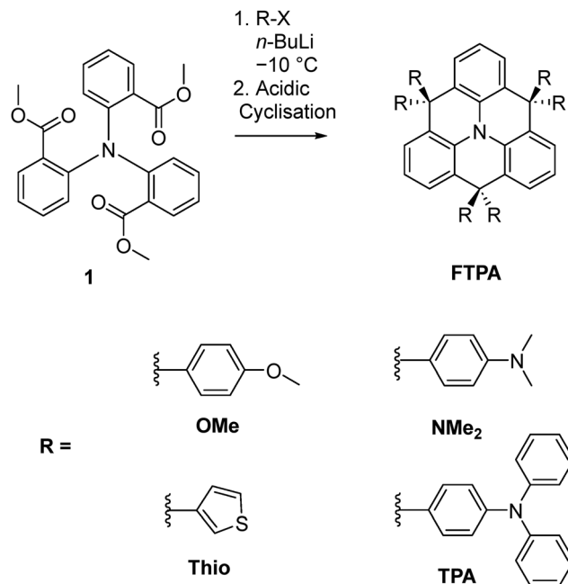
Scheme 1 Synthetic route to FTPA-OMe, FTPA-Thio, FTPA-NMe 2 and FTPA-TPA.
